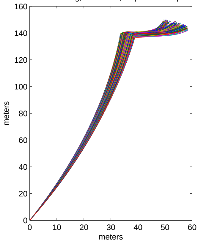
150.5m Mooring, 6m waves, 1s position snapshots
