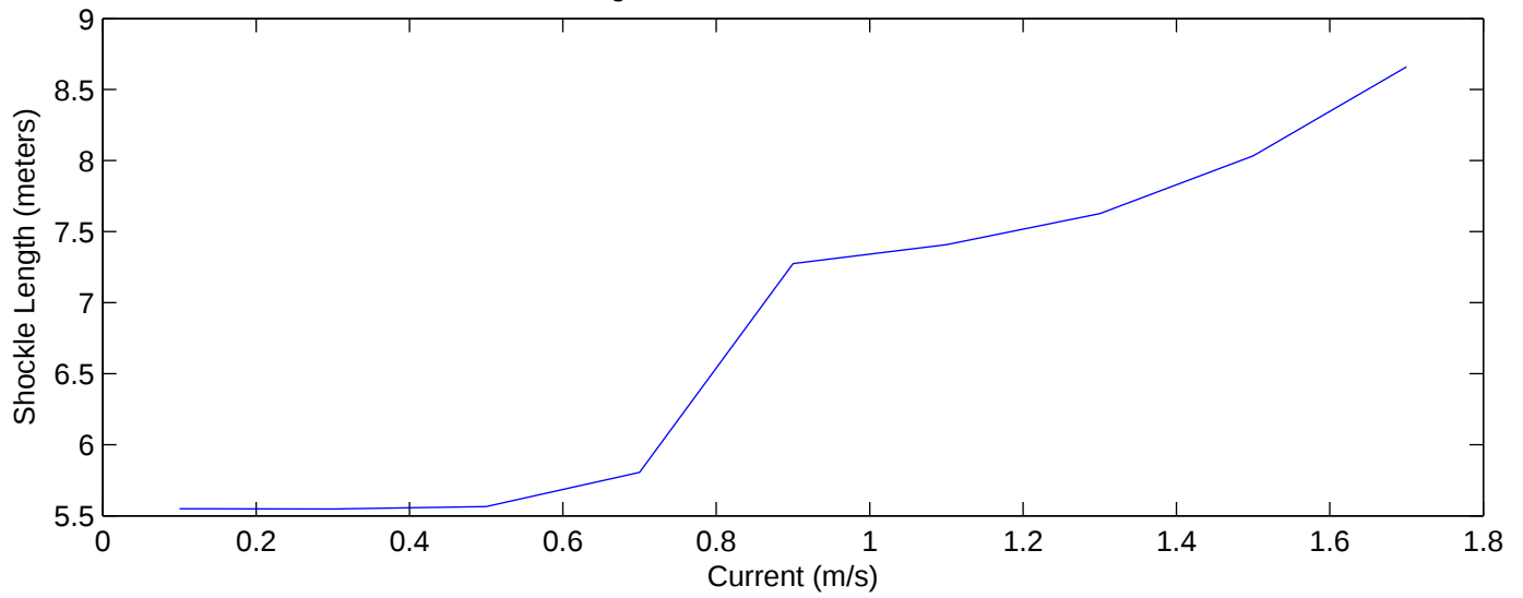
150m ESP Mooring Shockle Behavior in Constant Current Profile
