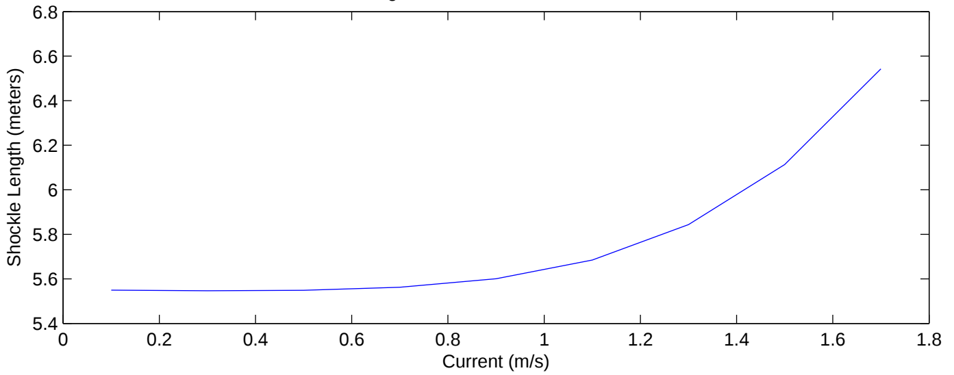
50m ESP Mooring Shockle Behavior in Linear Current Profile
