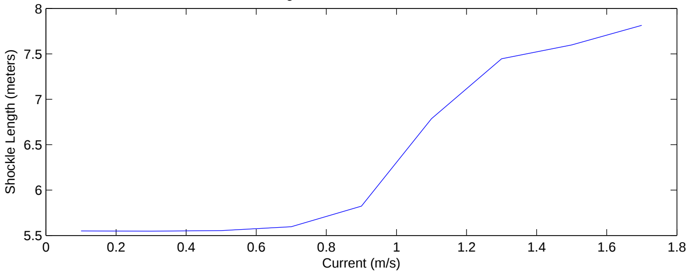
150m ESP Mooring Shockle Behavior in Linear Current Profile
