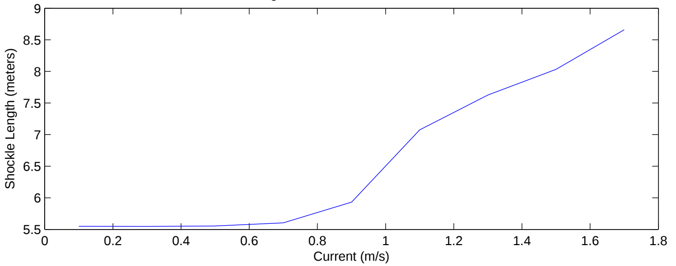
100m ESP Mooring Shockle Behavior in Constant Current Profile
