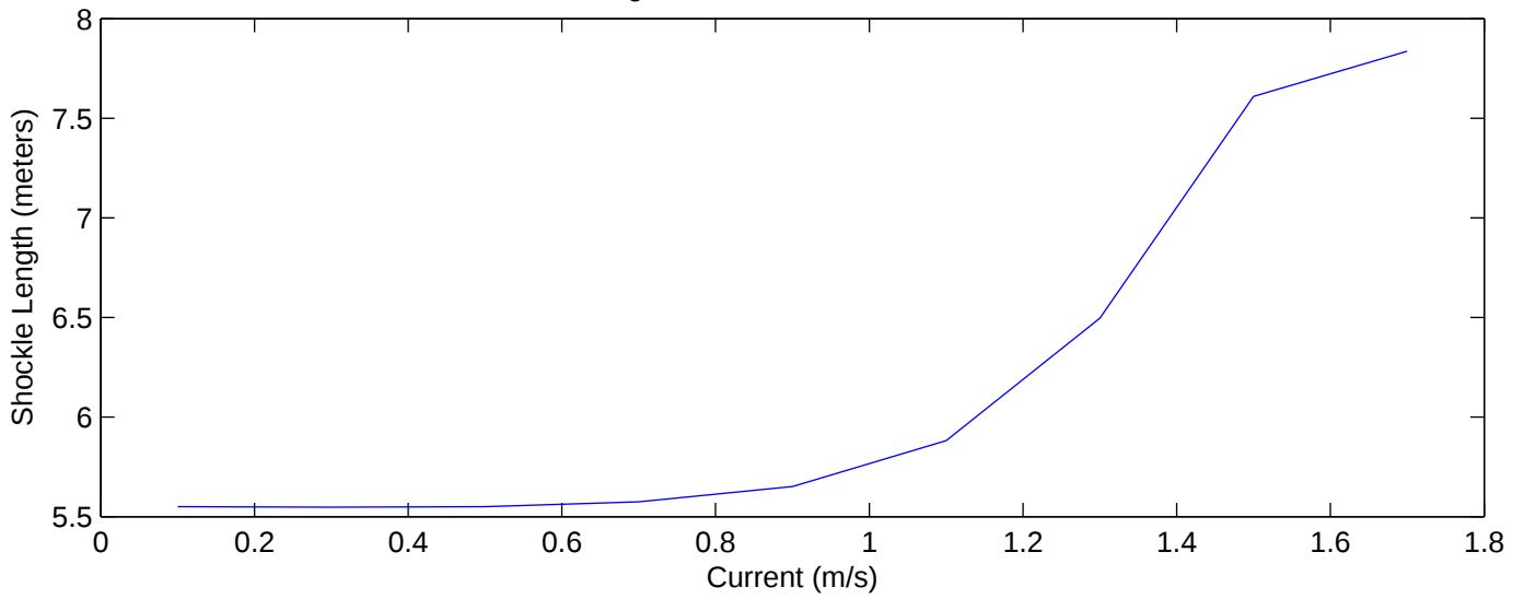
100m ESP Mooring Shockle Behavior in Linear Current Profile
