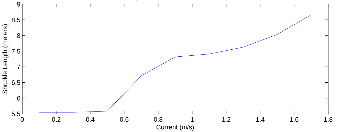
200m ESP Mooring Shockle Behavior in Constant Current Profile
