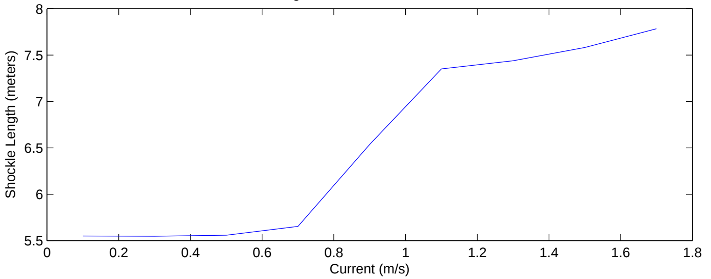
200m ESP Mooring Shockle Behavior in Linear Current Profile
