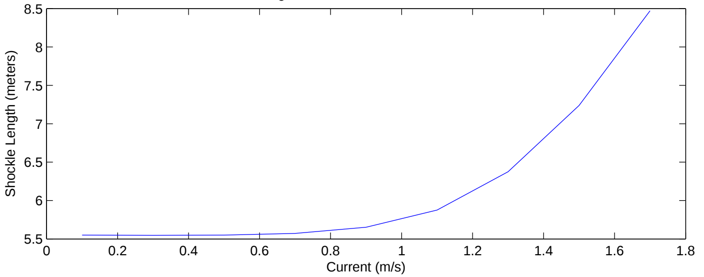
50m ESP Mooring Shockle Behavior in Constant Current Profile
