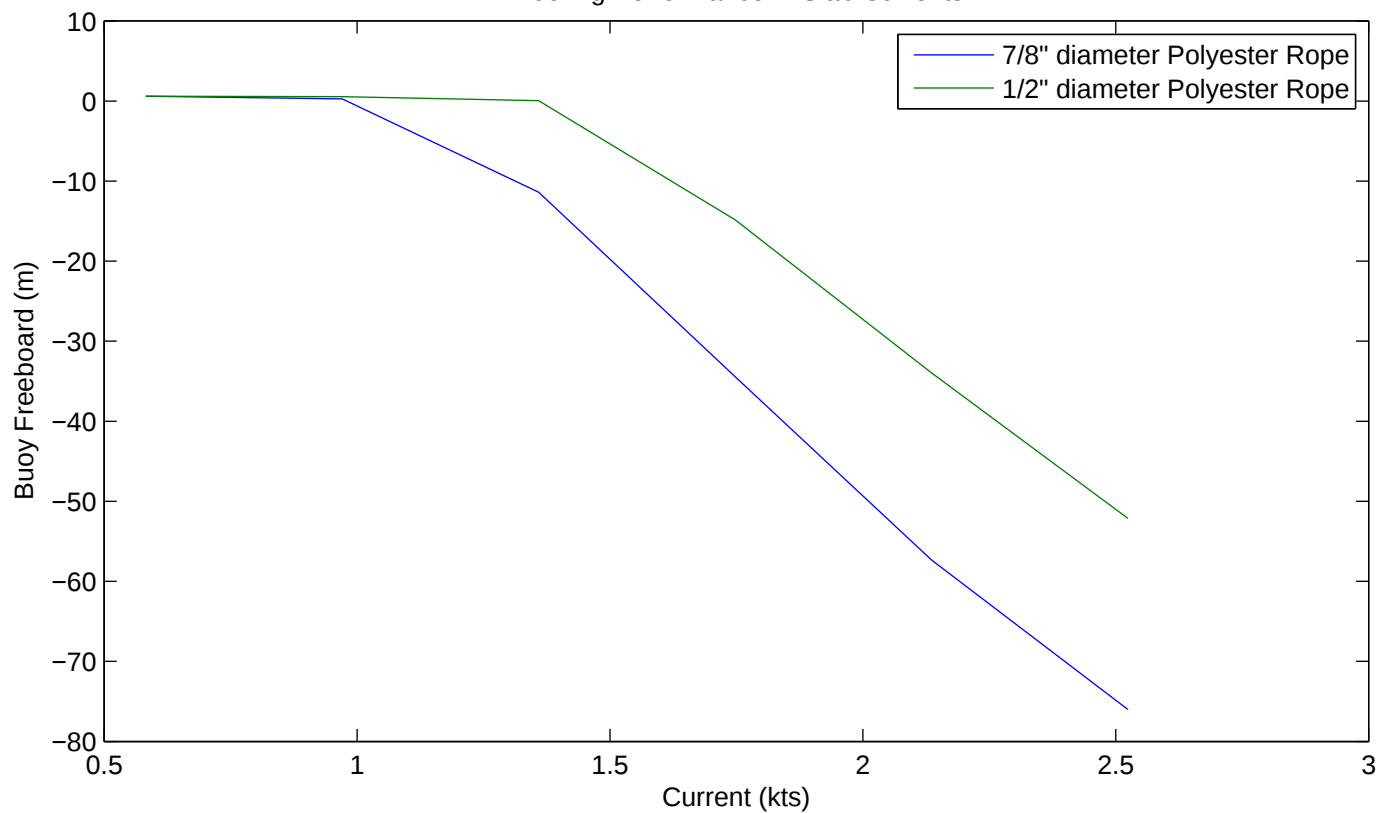
Mooring Performance in Slab Currents
