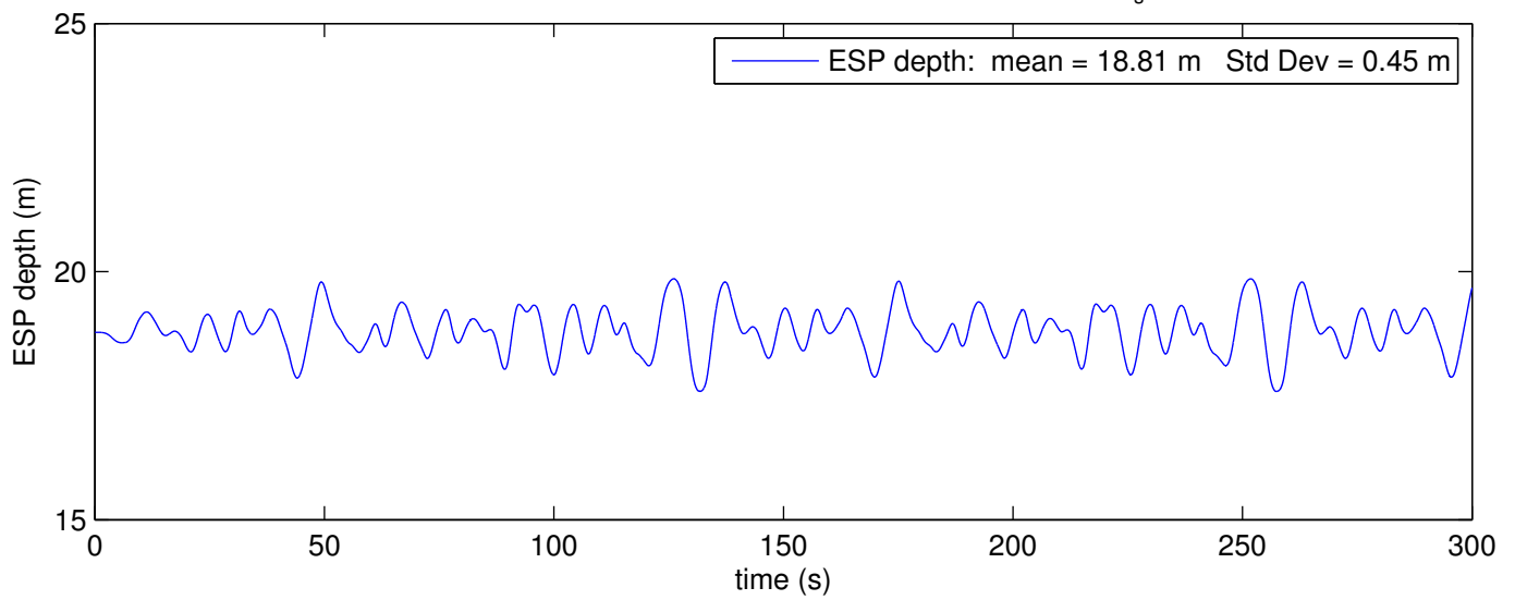
ESP Depth Results for Stiff Hose 44 lb Pig wet weight, 348 lb ESP wet weight H_s = 2 m Period = 14 s
