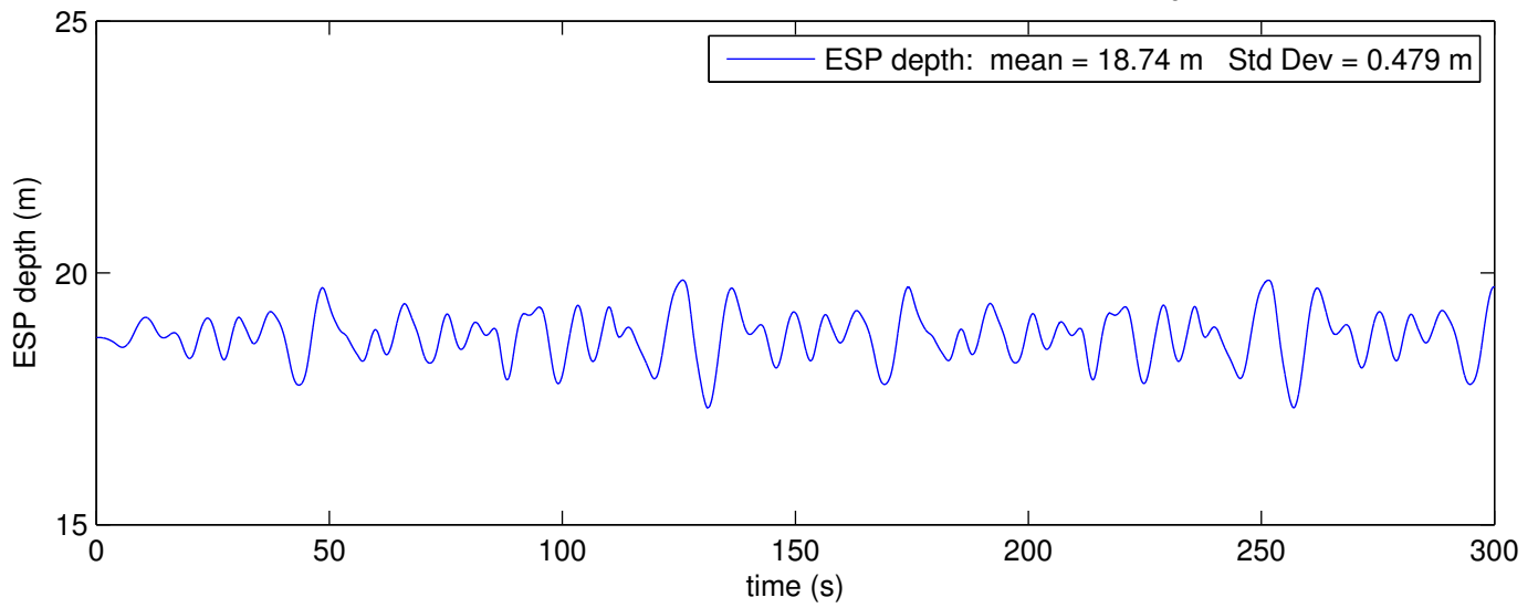
ESP Depth Results for Stiff Hose 440 lb Pig wet weight, -49.4 lb ESP wet weight H_s = 2 m Period = 14 s
