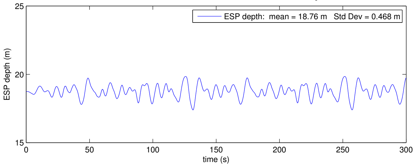
ESP Depth Results for Stiff Hose 220 lb Pig wet weight, 171 lb ESP wet weight H_s = 2 m Period = 14 s
