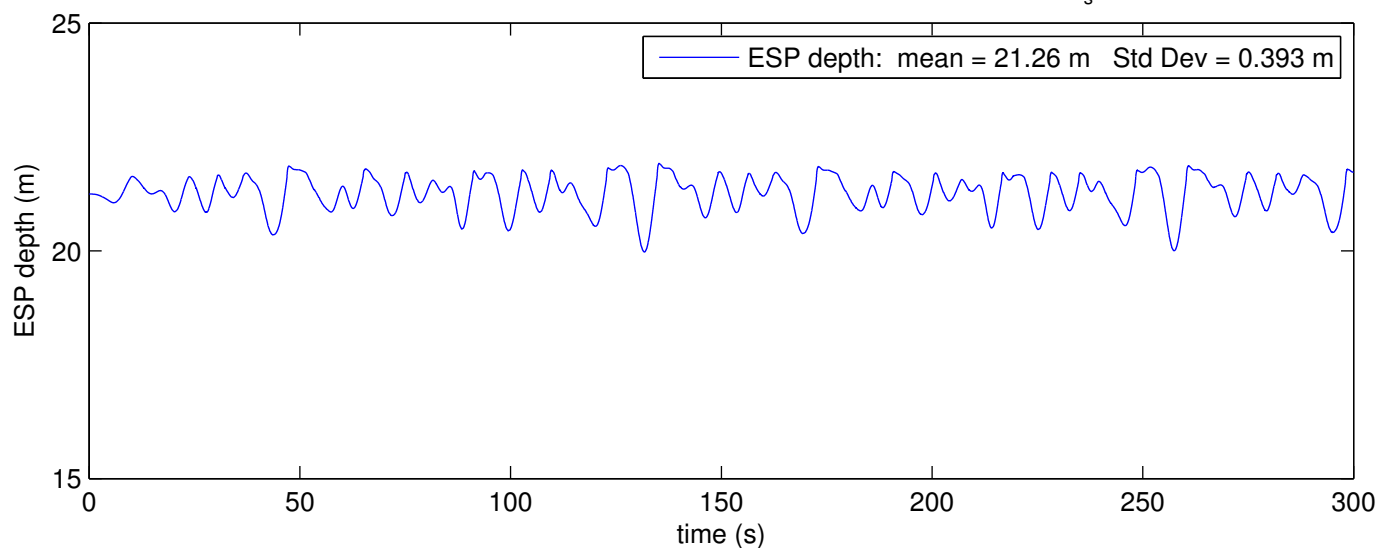
ESP Depth Results for Nominal Hose 440 lb Pig wet weight, -49.4 lb ESP wet weight H_s = 2 m Period = 14 s
