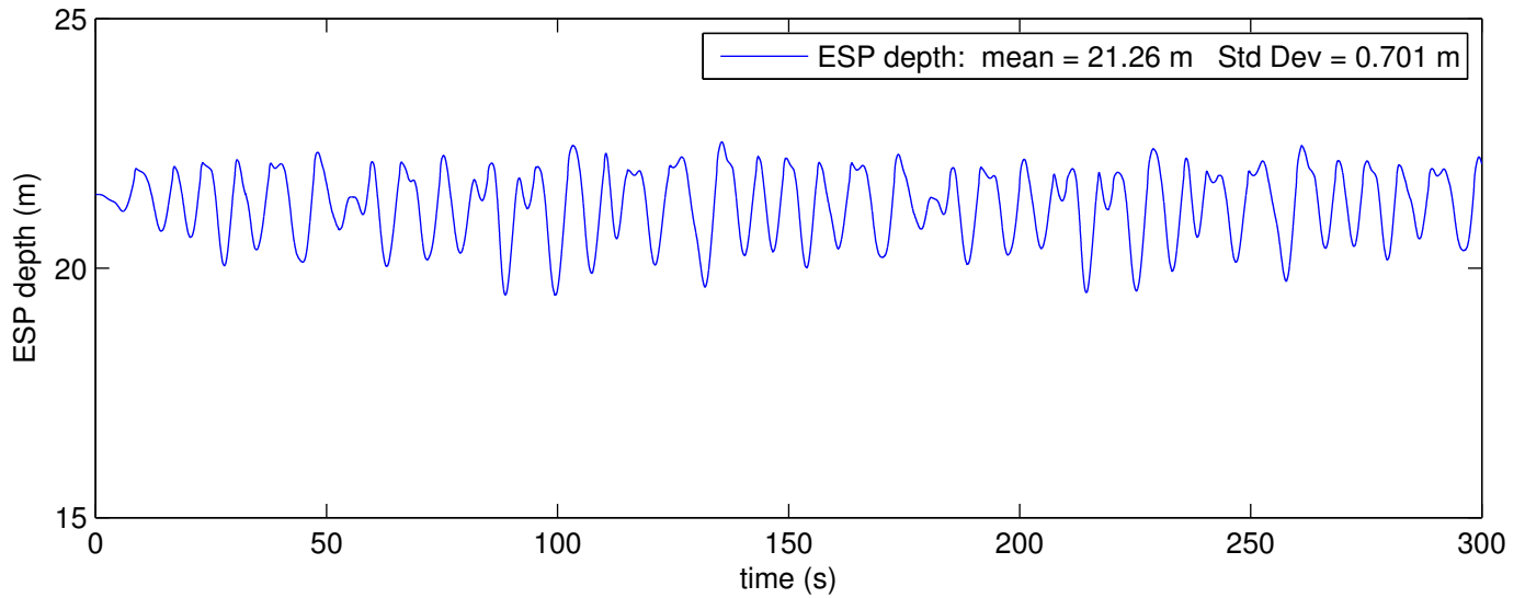
ESP Depth Results for Nominal Hose 440 lb Pig wet weight, -49.4 lb ESP wet weight H_s = 4.8 m Period = 9 s
