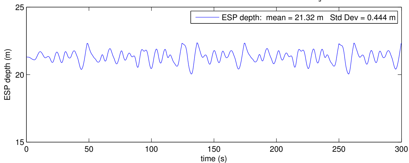
ESP Depth Results for Nominal Hose 220 lb Pig wet weight, 171 lb ESP wet weight H_s = 2 m Period = 14 s
