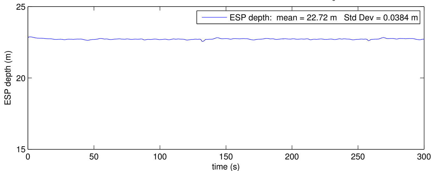
ESP Depth Results for Soft Hose 440 lb Pig wet weight, -49.4 lb ESP wet weight H_s = 2 m Period = 14 s
