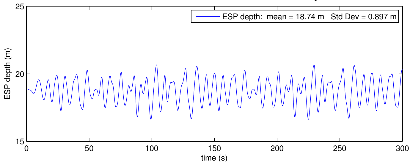
ESP Depth Results for Stiff Hose 440 lb Pig wet weight, -49.4 lb ESP wet weight H_s = 4.8 m Period = 9 s
