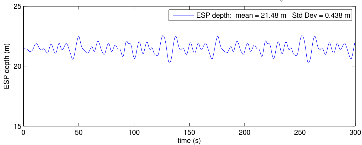
ESP Depth Results for Nominal Hose 44 lb Pig wet weight, 348 lb ESP wet weight H_s = 2 m Period = 14 s
