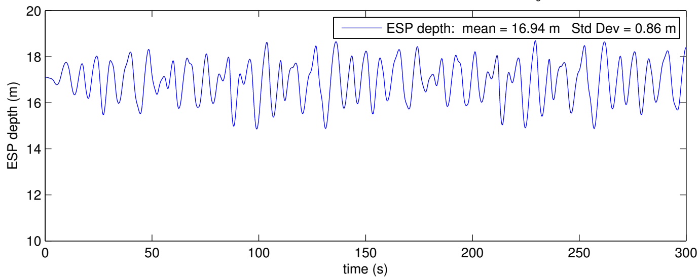
ESP Depth Results for Soft Hose 440 lb Pig wet weight, -49.4 lb ESP wet weight H_s = 4.8 m Period = 9 s
