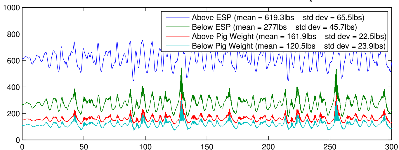
Dynamic Tension Results for Stiff Hose 44 lb Pig wet weight, 348 lb ESP wet weight H_s = 2 m Period = 14 s
