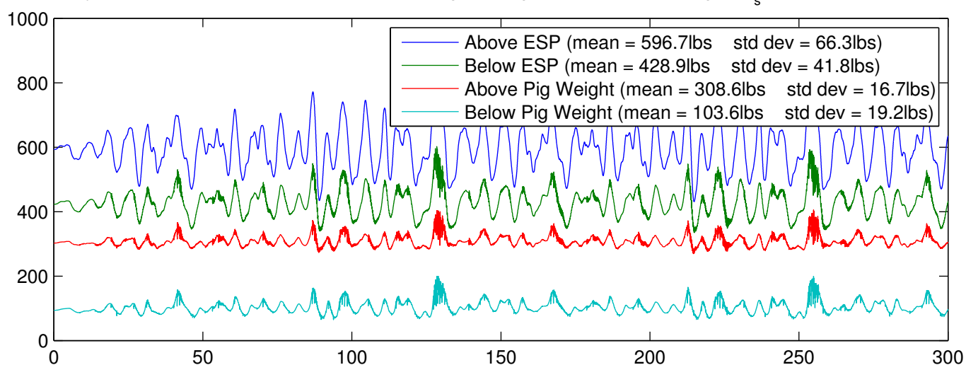
Dynamic Tension Results for Stiff Hose 220 lb Pig wet weight, 171 lb ESP wet weight H_s = 2 m Period = 14 s
