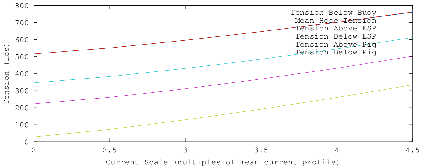
Static Tension Results for Soft Hose 220 lb Pig wet weight, 171 lb ESP wet weight
