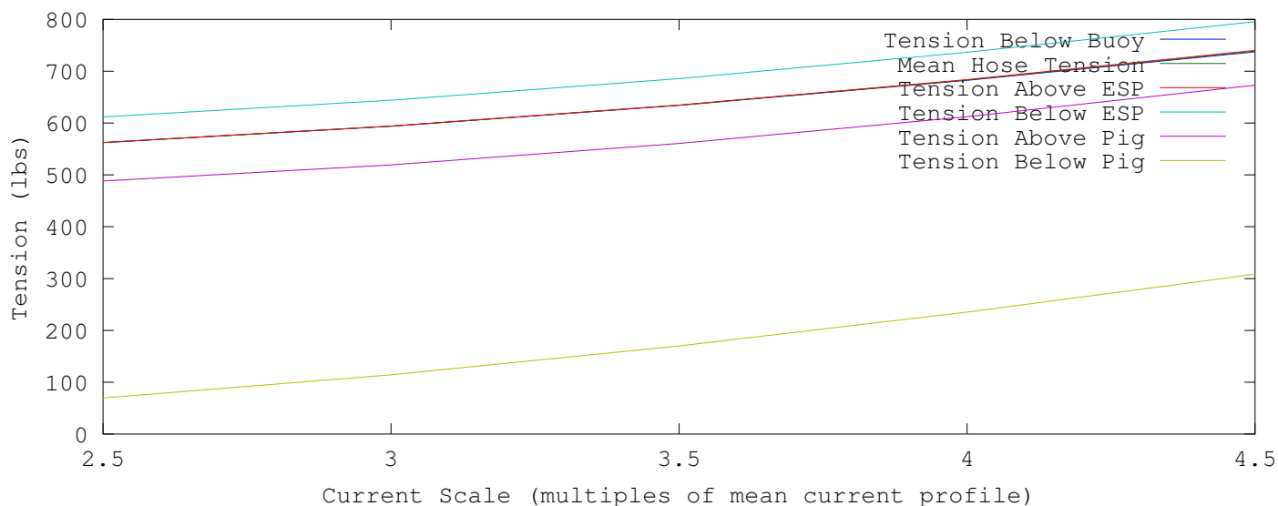
Static Tension Results for Nominal Hose 440 lb Pig wet weight, -49.4 lb ESP wet weight
