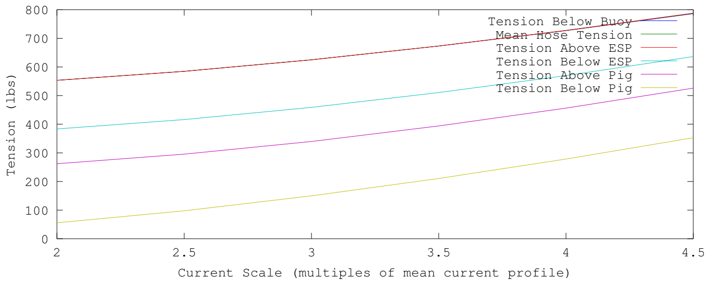
Static Tension Results for Nominal Hose 220 lb Pig wet weight, 171 lb ESP wet weight
