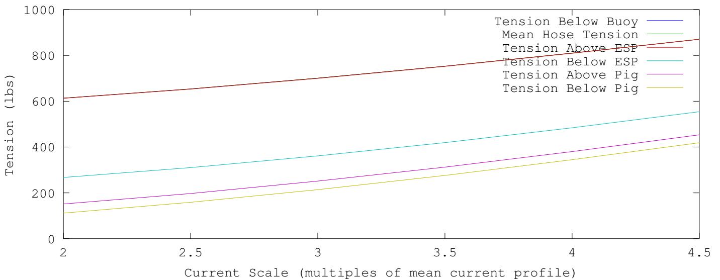
Static Tension Results for Stiff Hose 44 lb Pig wet weight, 348 lb ESP wet weight
