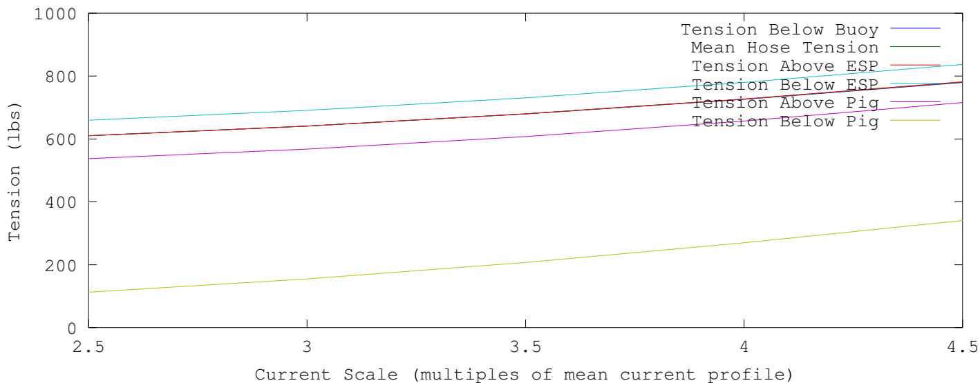
Static Tension Results for Stiff Hose 440 lb Pig wet weight, -49.4 lb ESP wet weight
