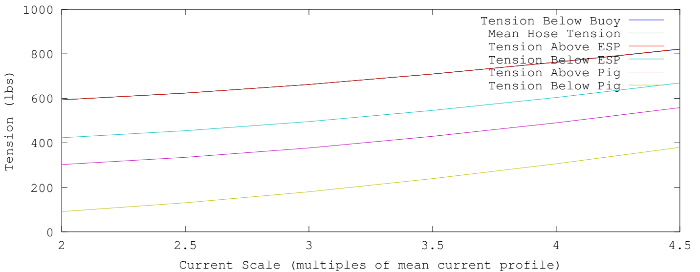
Static Tension Results for Stiff Hose 220 lb Pig wet weight, 171 lb ESP wet weight
