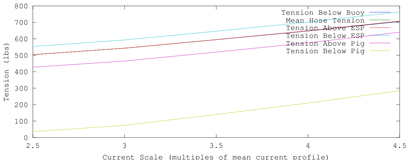
Static Tension Results for Soft Hose 440 lb Pig wet weight, -49.4 lb ESP wet weight
