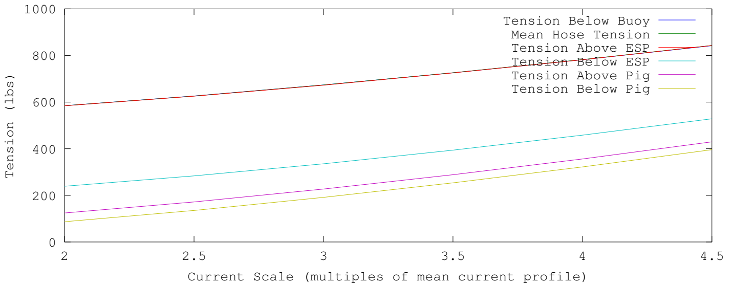
Static Tension Results for Nominal Hose 44 lb Pig wet weight, 348 lb ESP wet weight
