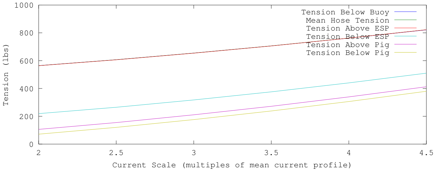
Static Tension Results for Soft Hose 44 lb Pig wet weight, 348 lb ESP wet weight
