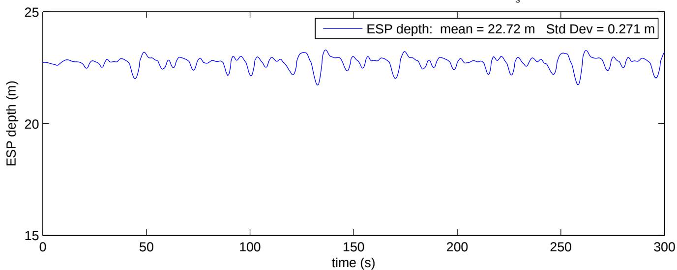
ESP Depth Results for Soft Hose 220 lb Pig wet weight, 171 lb ESP wet weight H_s = 2 m Period = 14 s
