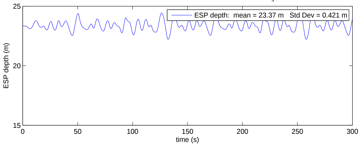
ESP Depth Results for Soft Hose 44 lb Pig wet weight, 348 lb ESP wet weight H_s = 2 m Period = 14 s
