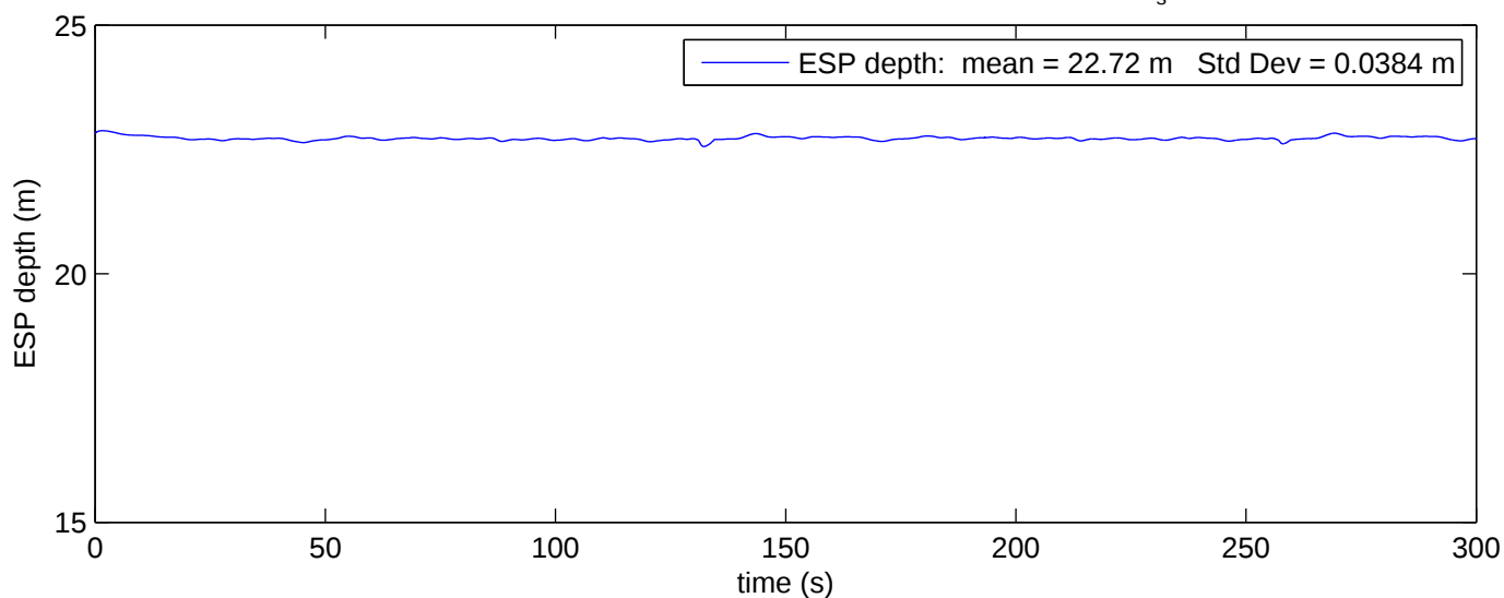
ESP Depth Results for Soft Hose 440 lb Pig wet weight, -49.4 lb ESP wet weight H_s = 2 m Period = 14 s
