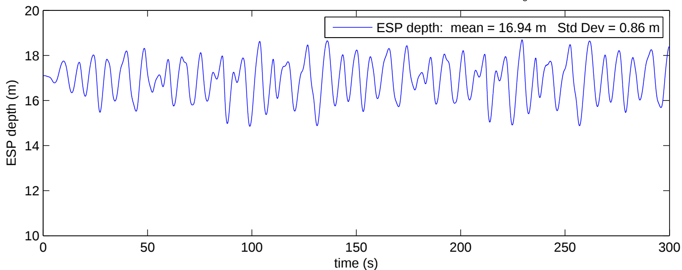
ESP Depth Results for Soft Hose 440 lb Pig wet weight, -49.4 lb ESP wet weight H_s = 4.8 m Period = 9 s
