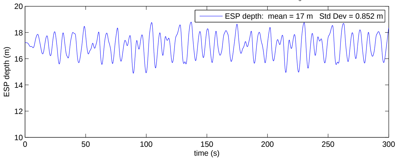
ESP Depth Results for Soft Hose 44 lb Pig wet weight, 348 lb ESP wet weight H_s = 4.8 m Period = 9 s
