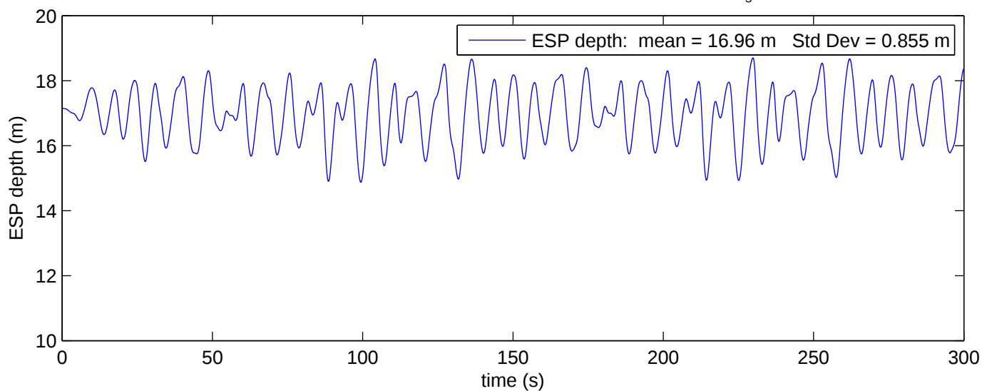
ESP Depth Results for Soft Hose 220 lb Pig wet weight, 171 lb ESP wet weight H_s = 4.8 m Period = 9 s
