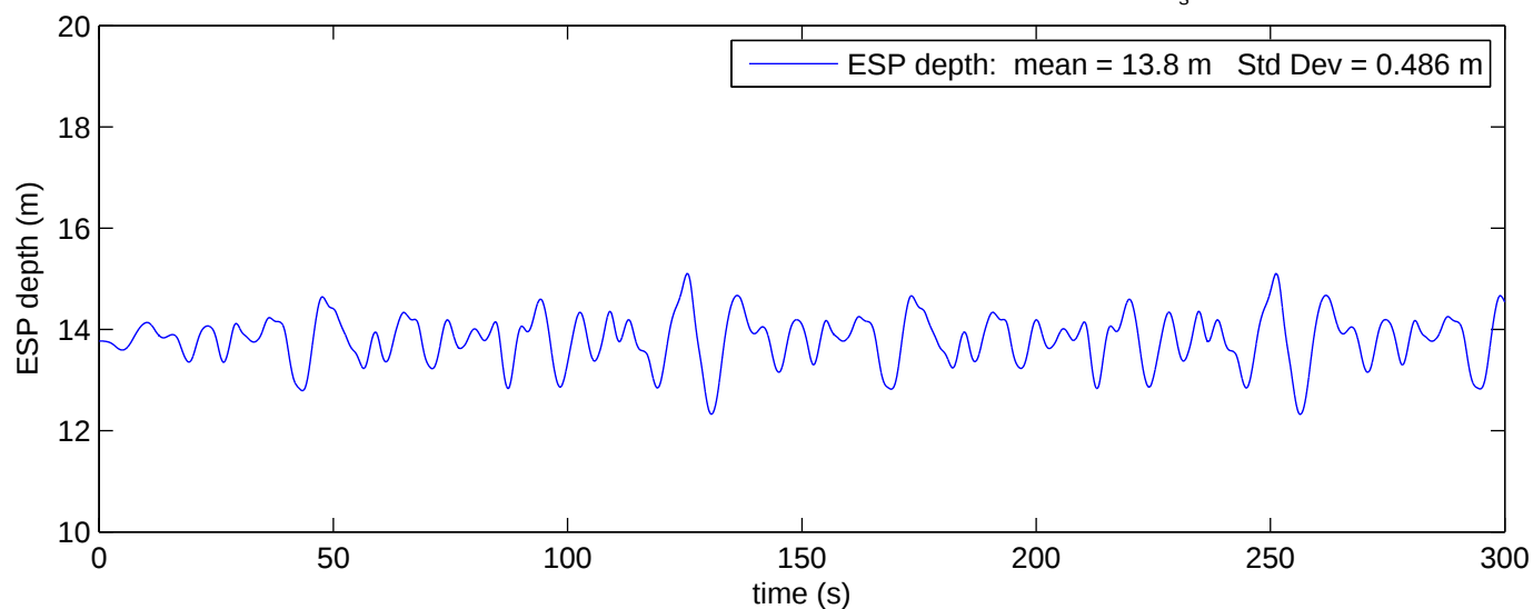
ESP Depth Results for Stiff Hose 440 lb Pig wet weight, -49.4 lb ESP wet weight H_s = 2 m Period = 14 s
