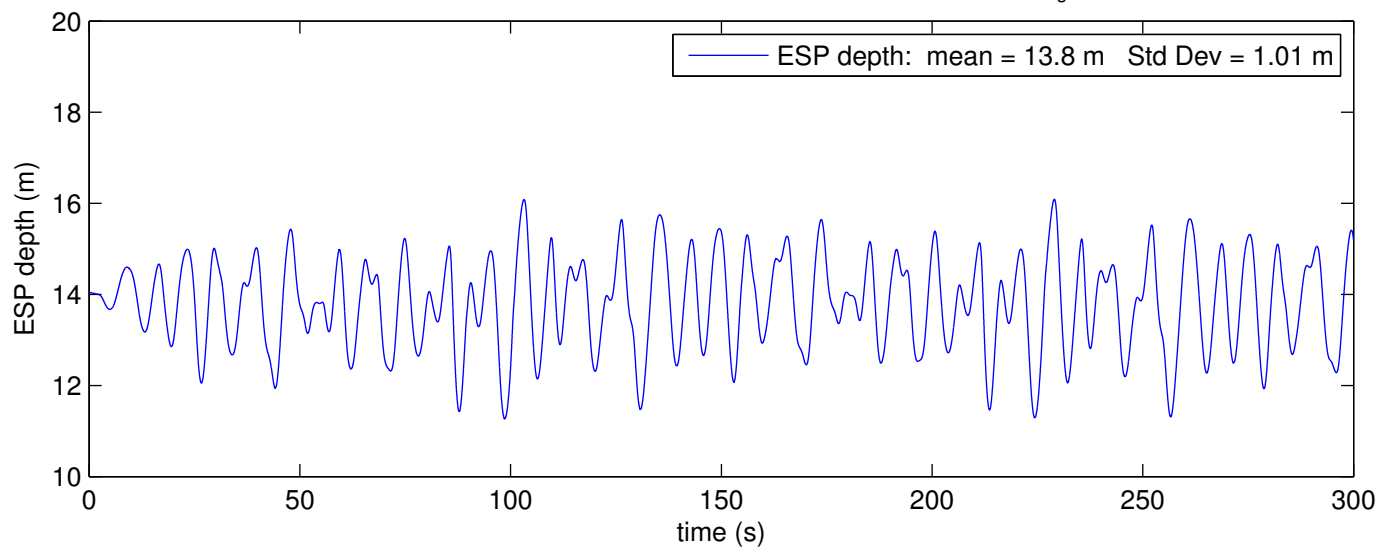
ESP Depth Results for Stiff Hose 440 lb Pig wet weight, -49.4 lb ESP wet weight H_s = 4.8 m Period = 9 s
