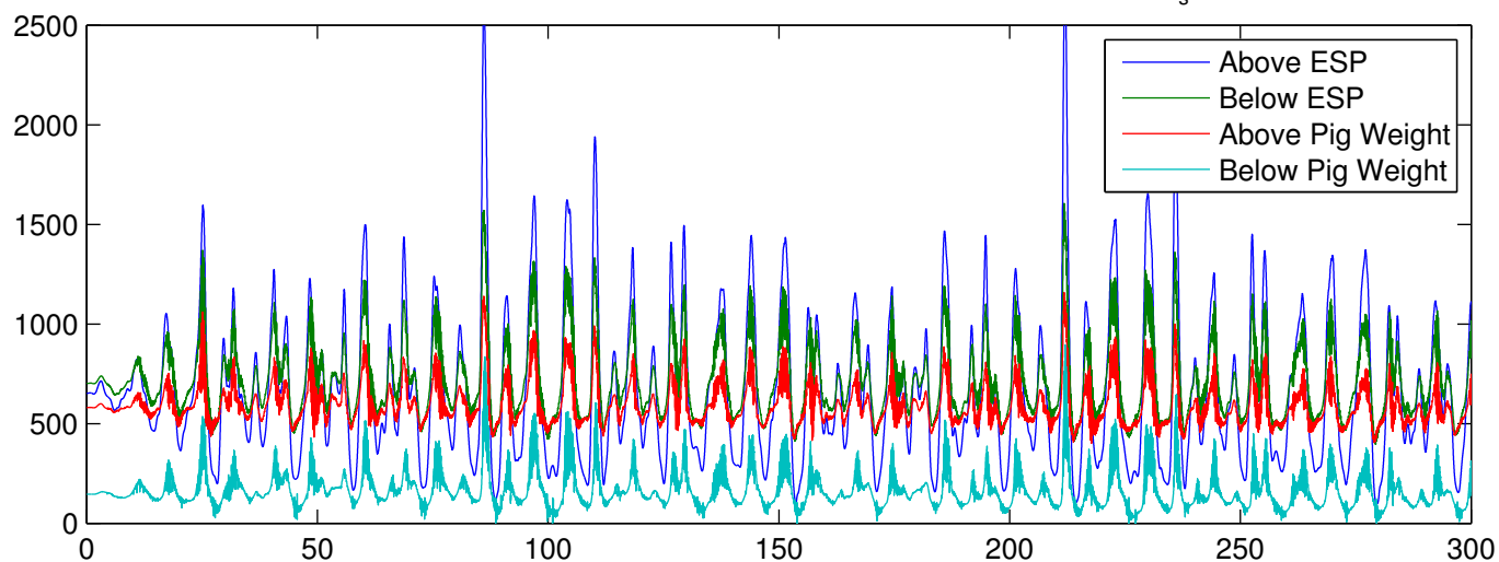
Dynamic Tension Results for Stiff Hose 440 lb Pig wet weight, -49.4 lb ESP wet weight H_s = 4.8 m Period = 9 s
