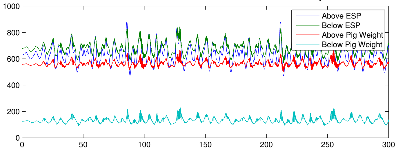
Dynamic Tension Results for Nominal Hose 440 lb Pig wet weight, -49.4 lb ESP wet weight H_s = 2 m Period = 14 s
