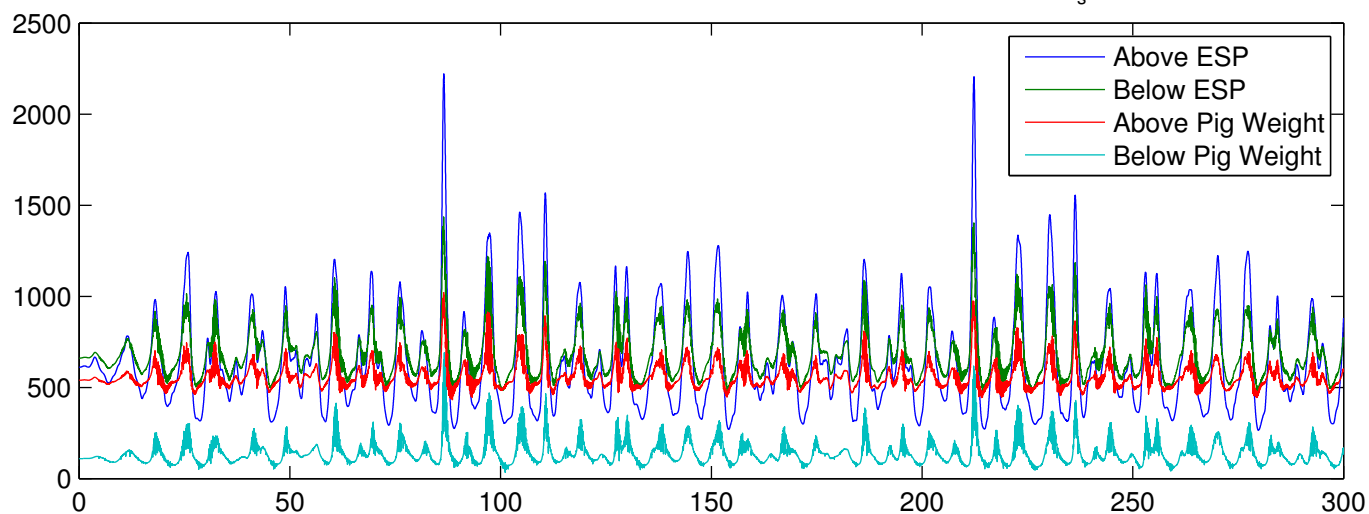
Dynamic Tension Results for Soft Hose 440 lb Pig wet weight, -49.4 lb ESP wet weight H_s = 4.8 m Period = 9 s
