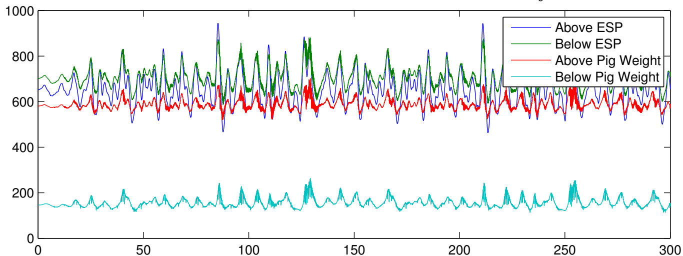
Dynamic Tension Results for Stiff Hose 440 lb Pig wet weight, -49.4 lb ESP wet weight H_s = 2 m Period = 14 s
