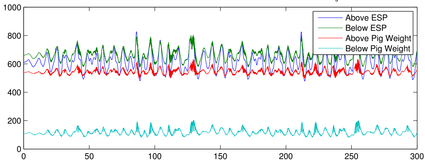
Dynamic Tension Results for Soft Hose 440 lb Pig wet weight, -49.4 lb ESP wet weight H_s = 2 m Period = 14 s
