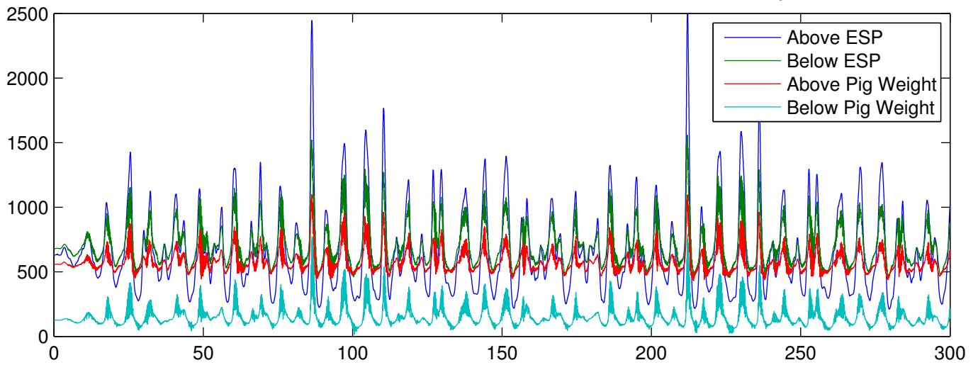
Dynamic Tension Results for Nominal Hose 440 lb Pig wet weight, -49.4 lb ESP wet weight H_s = 4.8 m Period = 9 s
