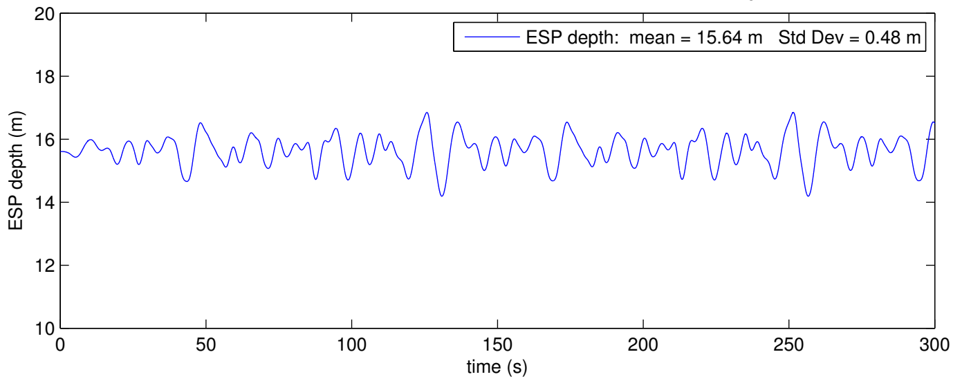
ESP Depth Results for Nominal Hose 440 lb Pig wet weight, -49.4 lb ESP wet weight H_s = 2 m Period = 14 s
