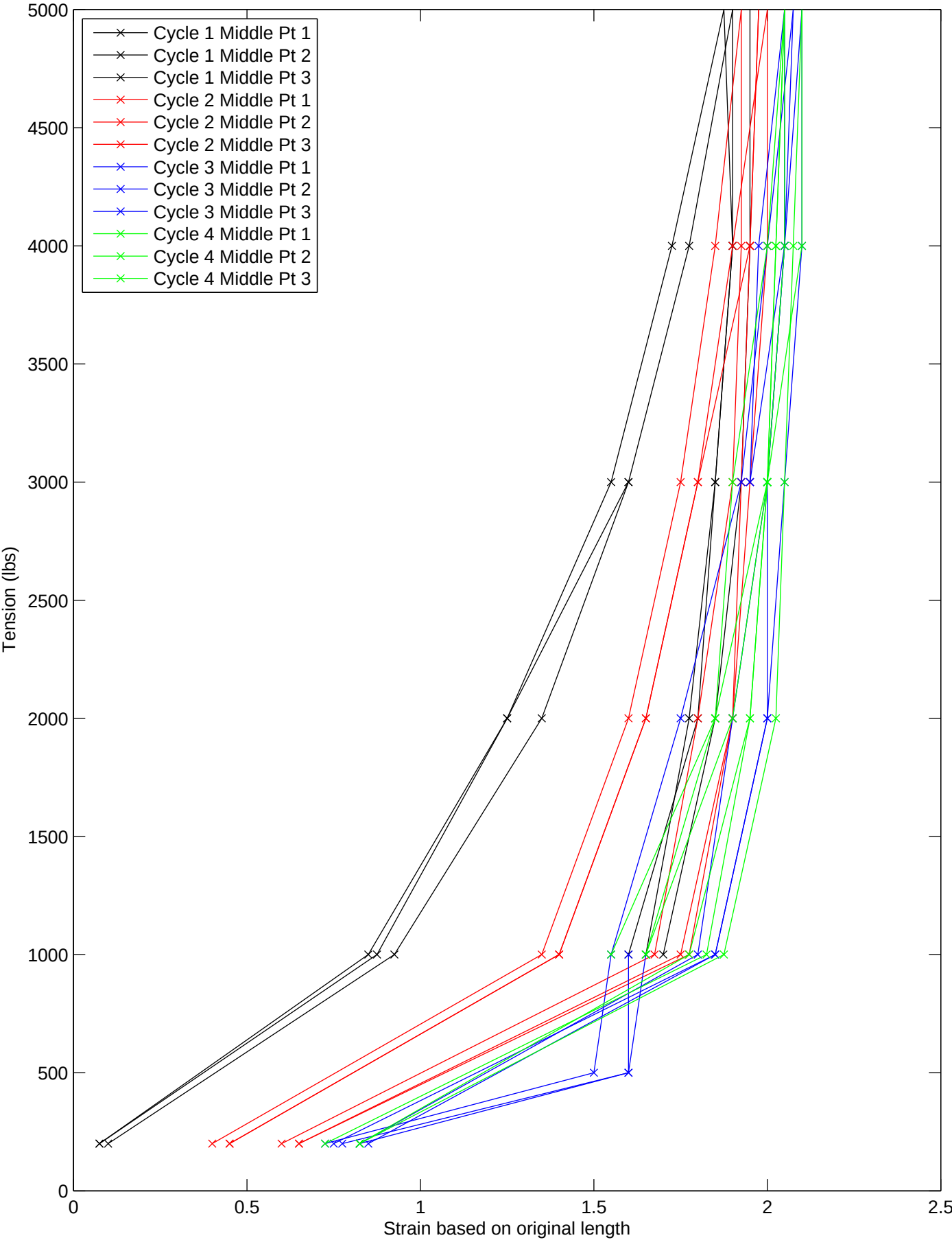
Tension-Strain Curves for Fully Compliant Section
