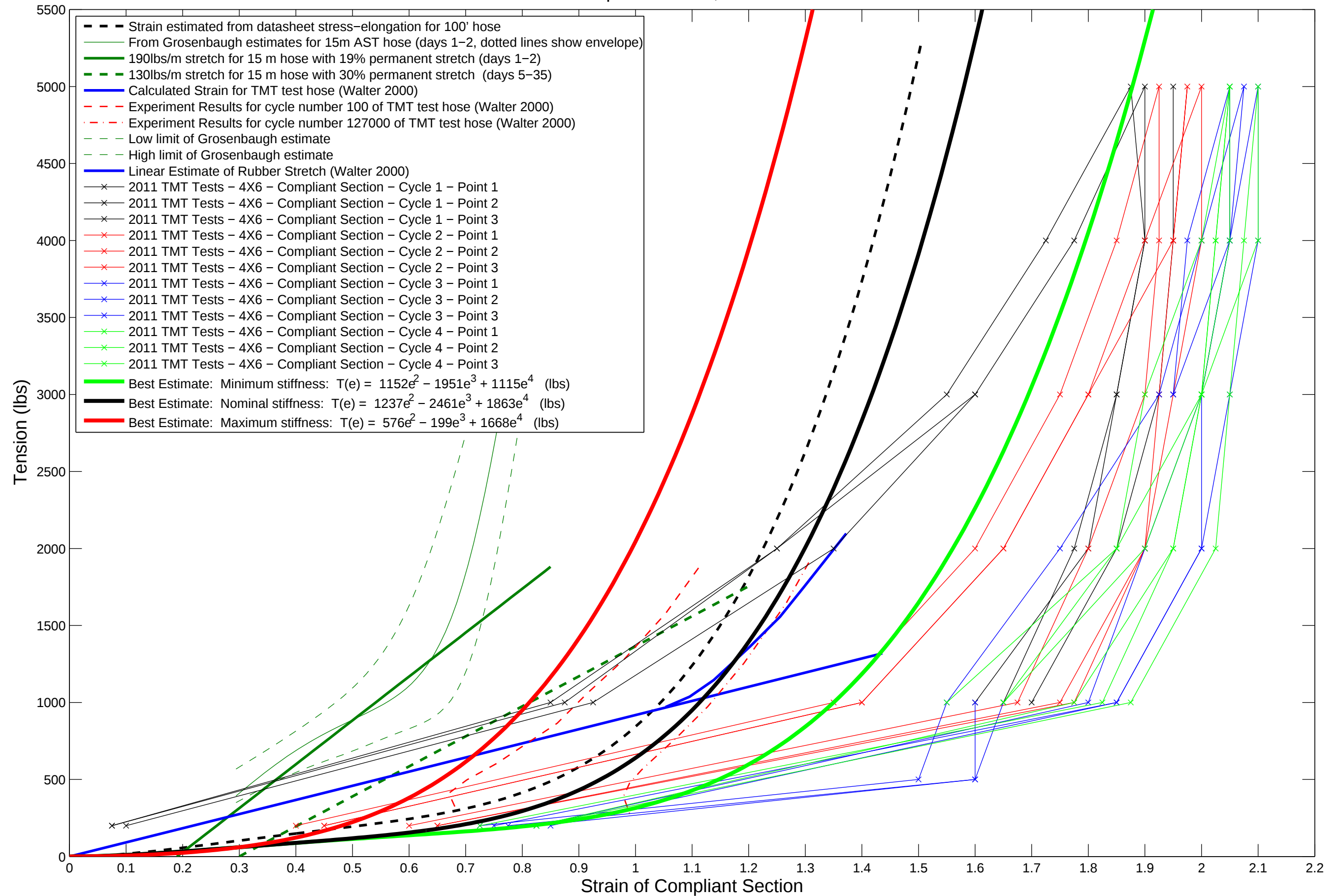
Stress-Strain of Compliant section, estimated from various tests
