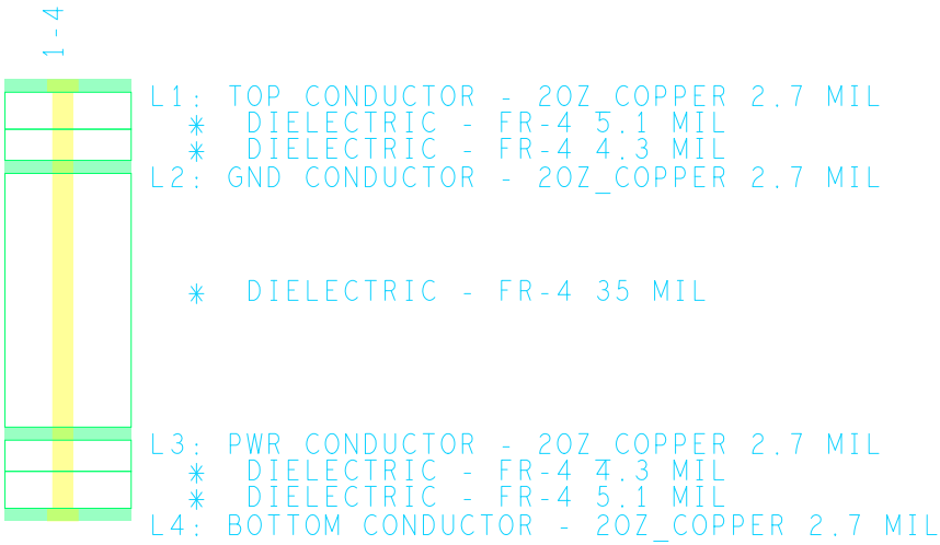
DESIGN CROSS SECTION CHART TOTAL THICKNESS 64.6 MIL
