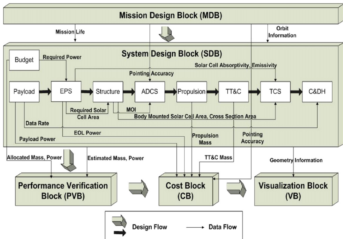
Fig. 1. SEDT architecture.
