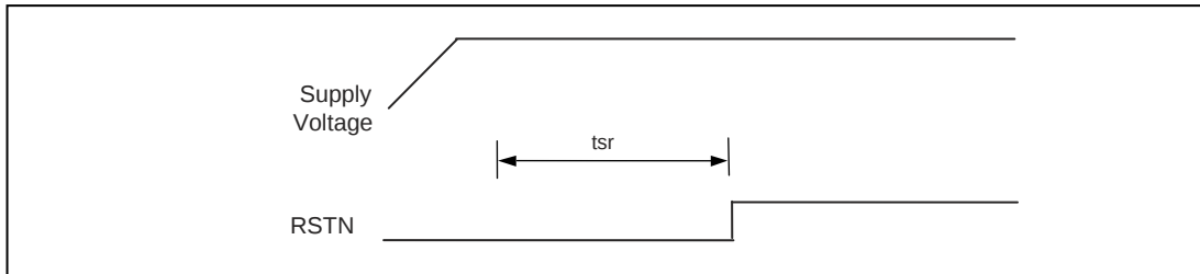
Figure 12. Reset Timing
