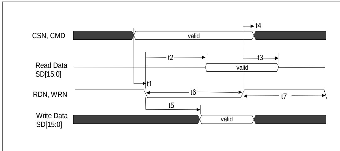
Figure 10. Asynchronous Cycle
