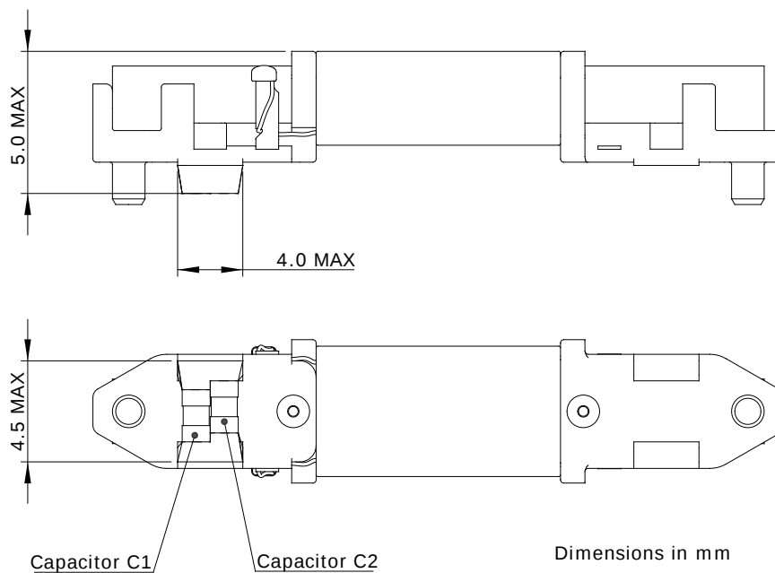
Figure 6 Dimensions, part 013-1024
