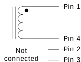
Figure 1 Electrical connections, 012-1704
