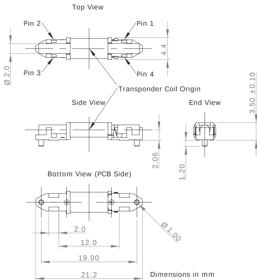
Figure 2 Dimensions, part 012-1704
