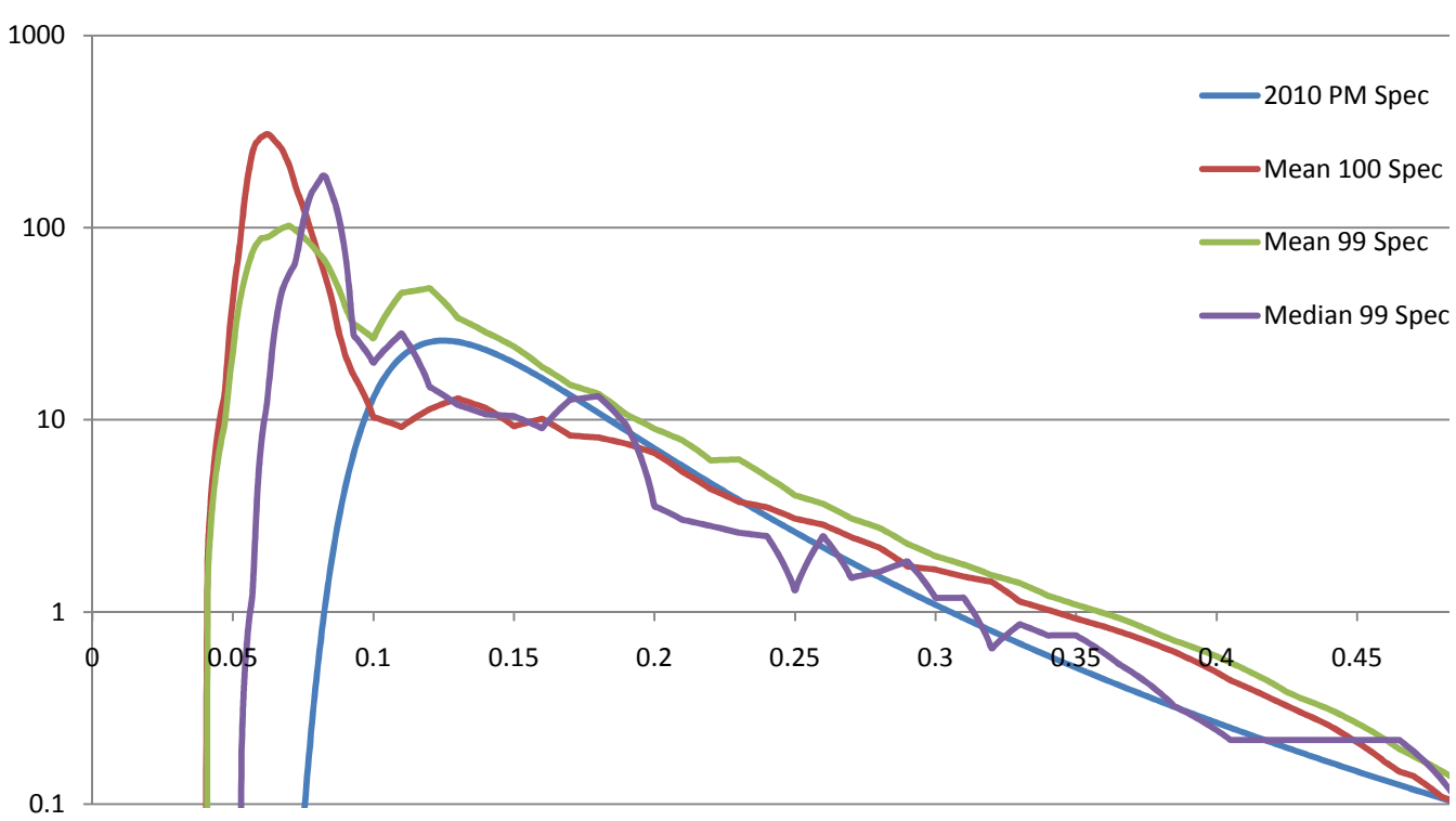
Spectral Density (ft 2 / Hz) dB Scale
