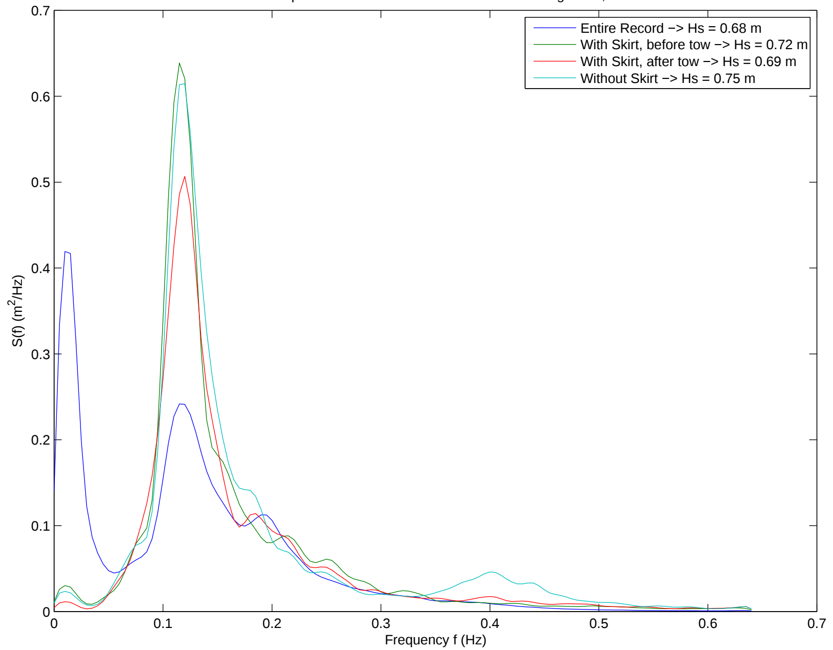
PSD comparisons of WaveRider Heave Motions – August 12, 2010
