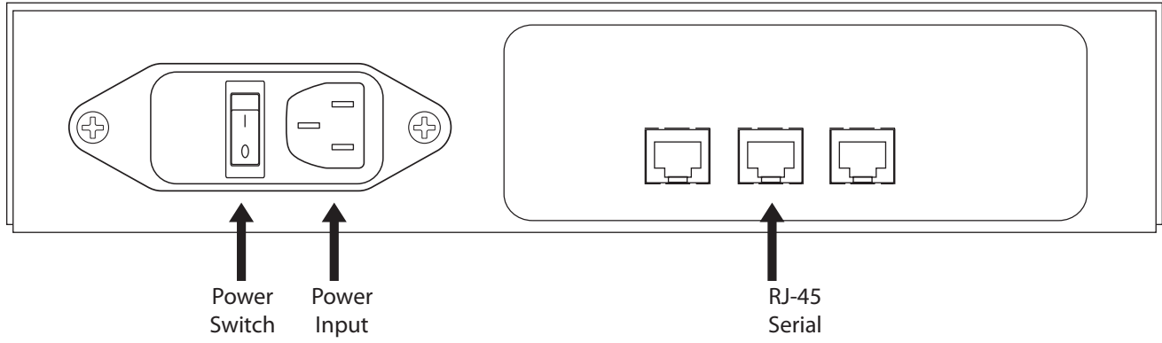
Digi Connect ES - Front
