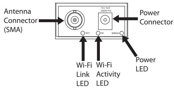
Digi Connect Wi-SP - Back
