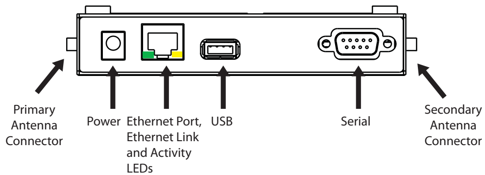
ConnectPort X4 - Front panel
