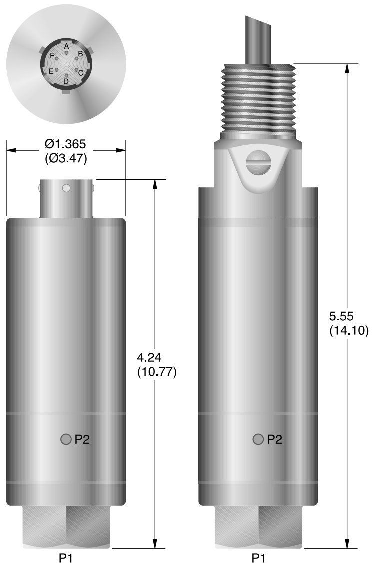
Figure 9.2—PPTR Case Outline
