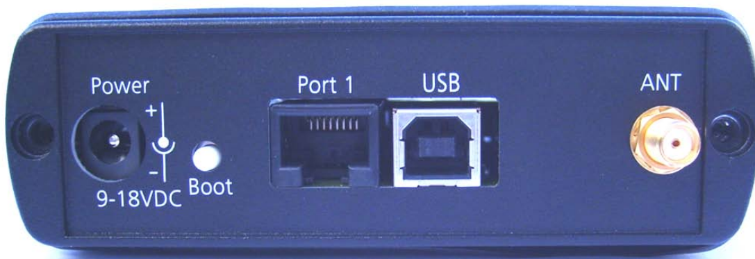
Figure 2: Rear panel
