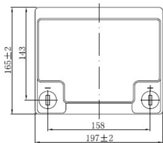
Exterior drawing for PS-12400NB
