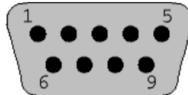
Figure 5 - SGI 9-Pin Connector
