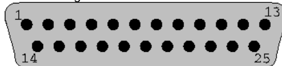
Figure 3 - RS-422 Connector
