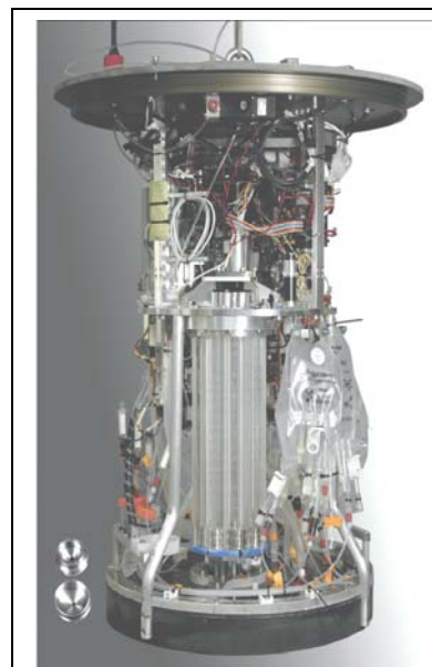
Figure 1. Second generation ESP instrument (16" d x 30" h). bottom left: puck magnified ~2x relative to those loaded in the carousel. See also: http://www.mbari.org/ESP/esp2G_compare.htm
