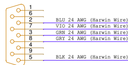
DB9 PLUG.MP Male Pins
