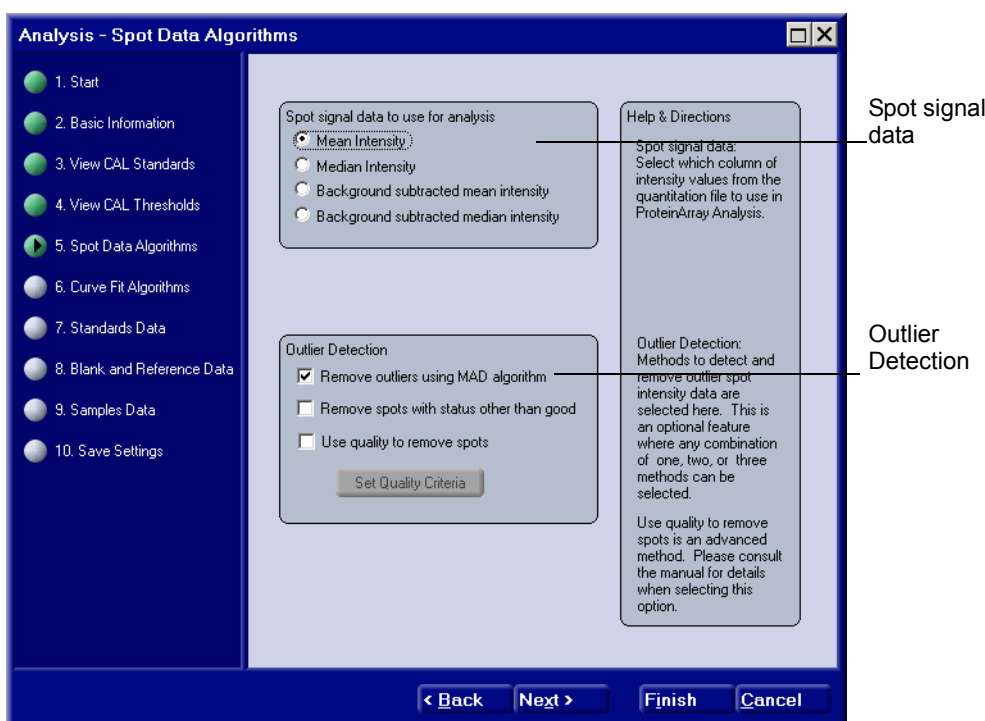
Figure 2-7 Analysis - Spot Data Algorithms Window
