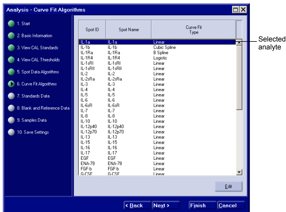
Figure 3–8 The Curve Fit Algorithms Window
