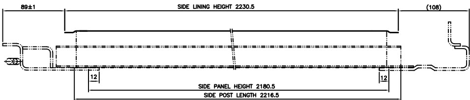
SECTION B-B SCALE 1:5
