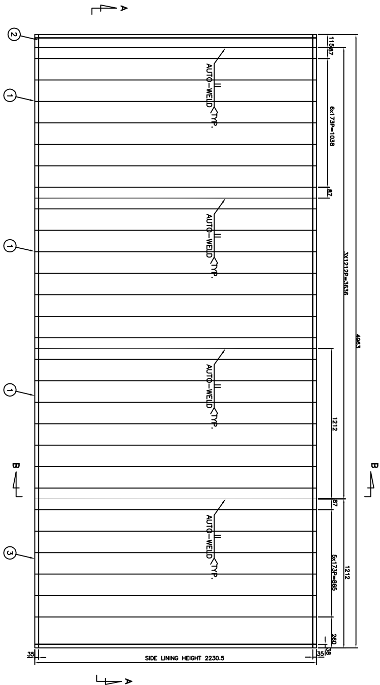
R/H SIDE LINING VIEW
