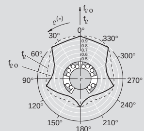
Open type
