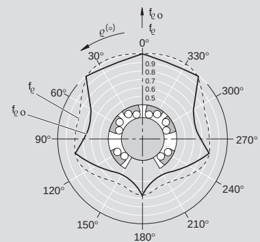
Open type
