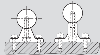
Conventional flanged design
