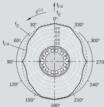
Closed type
