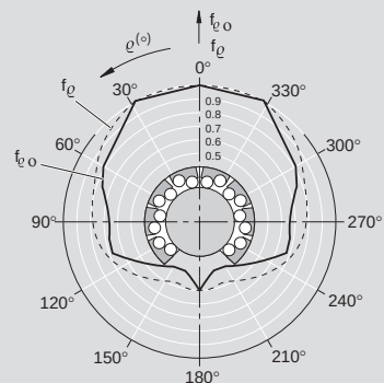
Open type
