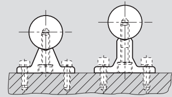
Conventional flanged designs
