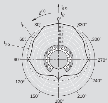
Open type
