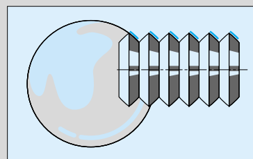
Recirculating roller screw Grooved rollers are the basis of « SV / BV / PV » recirculating roller screws.
