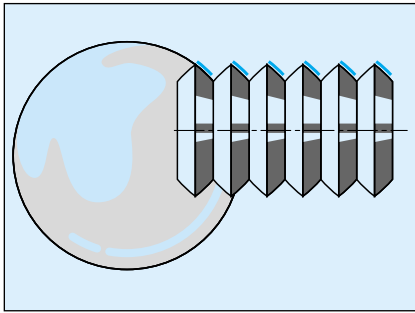
Grooved rollers are the basis of SV/BV/PV recirculating roller screws.
