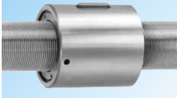
Preloaded cylindrical nut
