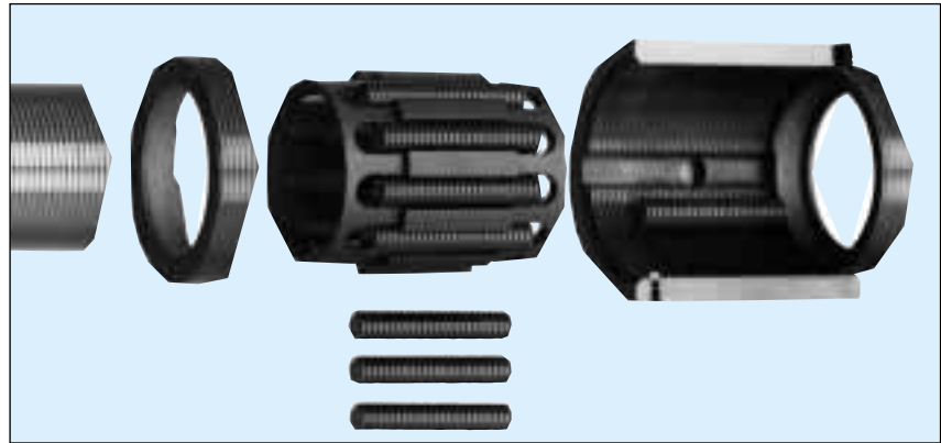
Grooved rollers are the basis of SV/BV/PV recirculating roller screws.
