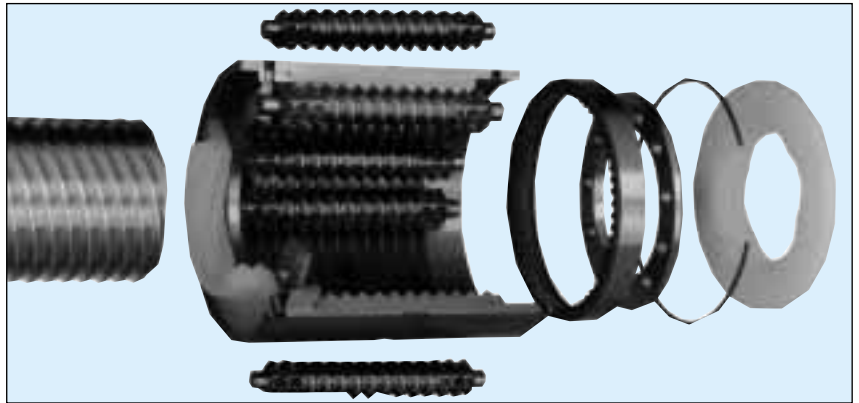
Threaded rollers are the basis of SR/BR/TR/PR planetary roller screws.
