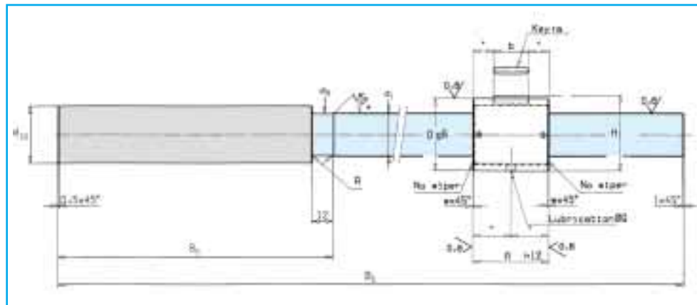
Recirculating roller screw
