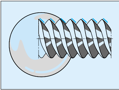
Threaded rollers are the basis of SR/BR/TR/PR planetary roller screws.
