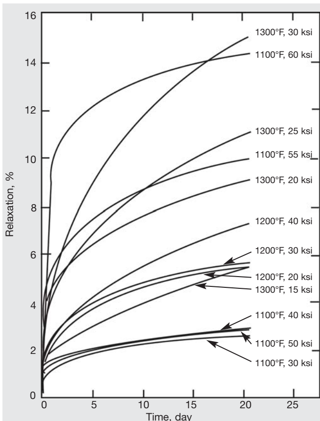
Figure 27. Relaxation of springs cold-coiled from triple-heat-treated Spring Temper wire (2100°F/2 hr, A.C., + 1550°F/24 hr, A.C., + 1300°F/20 hr, A.C.).
