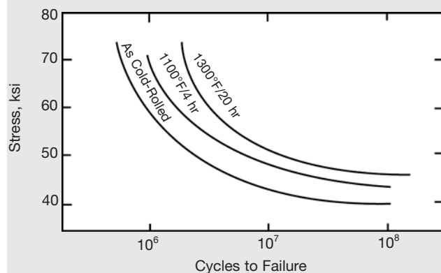
Figure 32 - Fatigue strength of cold-rolled Spring-Temper strip (tested in completely reversed bending at room temperature).
