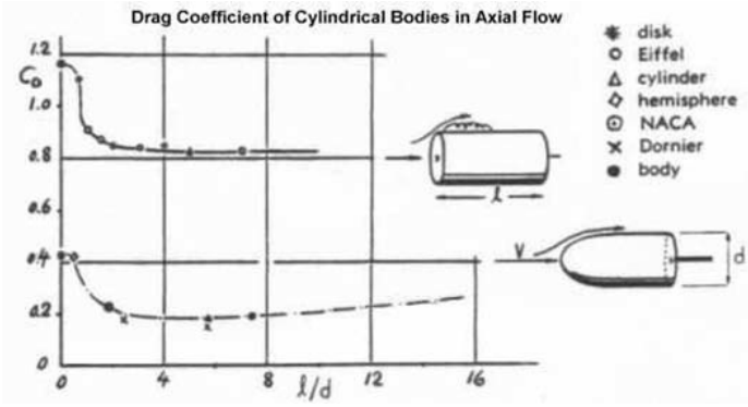
Fig. 14. Drag coefficient graph for applying to the AUV body
