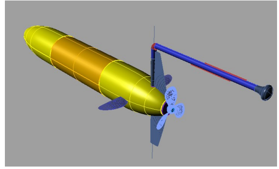
Fig. 16. Long mast replied in navigation mode
