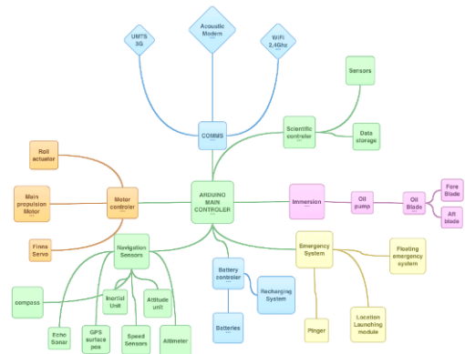
Fig. 10. Functional graphic of the operative modules and microprocessor
