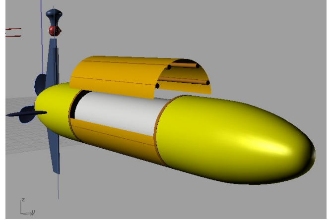
Fig. 9. Top cover open for battery mid section access
