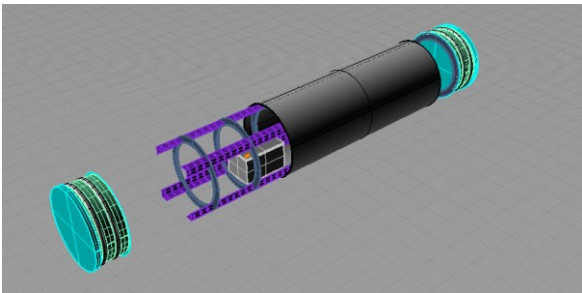
Fig. 8. Mid section assembly showing internal structure and closing
