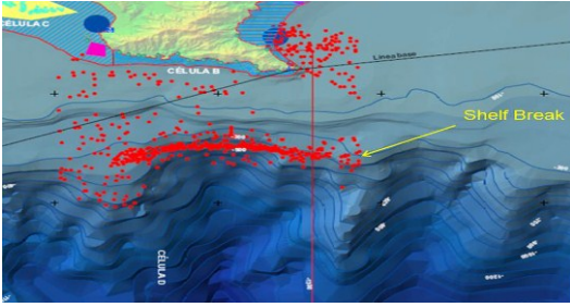
Fig. 7. Shelf break area off cape Tinoso
