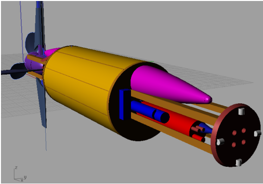
Fig. 17. Aspect of the nose section showing the bladder floating device and scientific instruments
