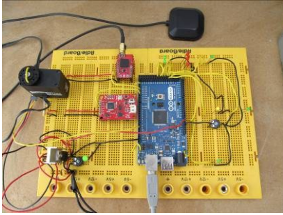
Fig. 4. Protoboard.
