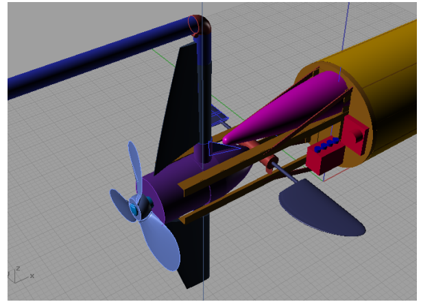
Fig. 12. Aft section detail showing foils actuators motor and Sampler and sensor
