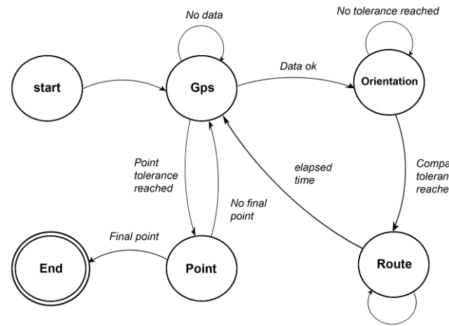
Fig. 2. AUV's states.
