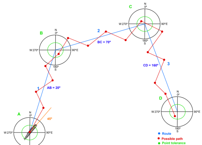
Fig. 3. AUV route example.
