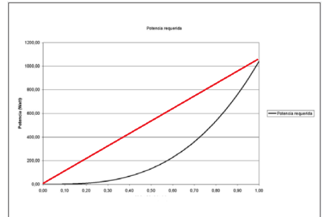
Fig. 15. Power-thrust function and linearization as upper limit
