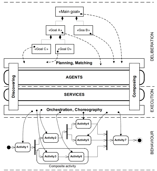
Fig. 3. Service-oriented agent-based architecture
