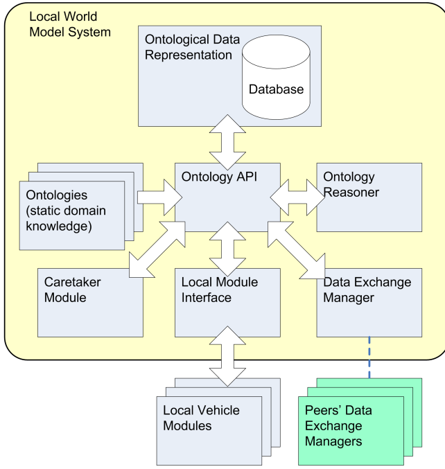
Fig. 1. Proposed World Model Architecture
