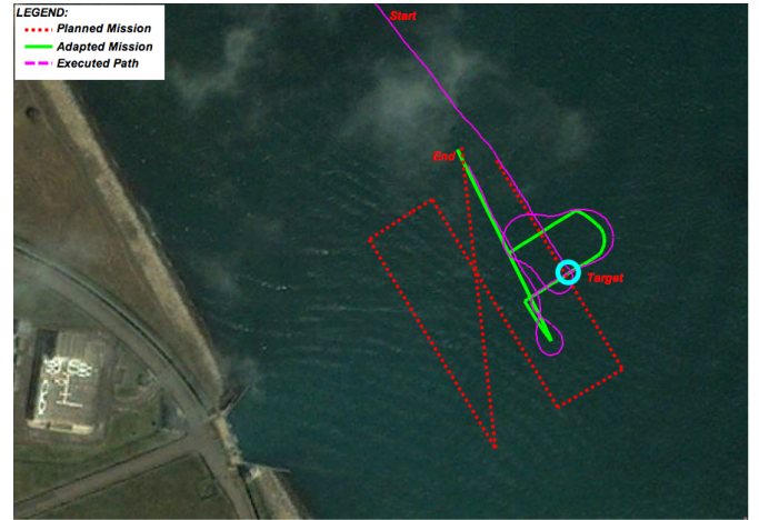
Fig. 6. AUV path during the adaptive mission at Tuas, Singapore field experiment in August 2012. Red dotted line shows the initial planned survey path. When a simulated target is detected, the mission was interrupted and re-planned (green solid line) to re-visit the target before proceeding to the end point.
