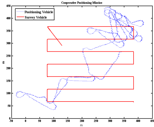
Fig. 4. Simulation results show the resultant path generated by the positioning AUV (blue dotted line) to minimize the position errors of the Survey AUV (red solid line).
