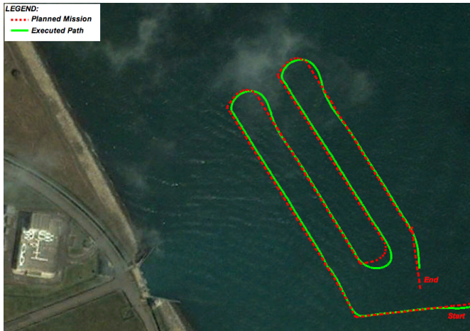
Fig. 5. Planned (red dotted line) and executed (green solid line) survey paths by the STARFISH AUV during the Tuas, Singapore field experiment in August 2012.
