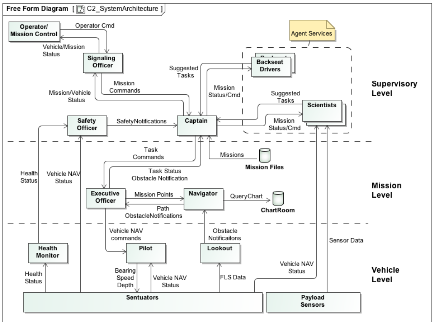
Fig. 2. Overview of the Command and Control System.
