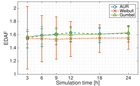
Fig. 20. EDAF with CI for cylinder with T_n = 5.0[s] . 40 seeds are used for each simulation time.
