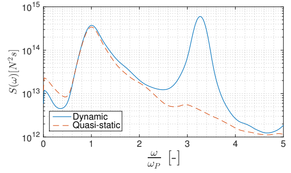
Fig. 9. Dynamic and quasi-static response spectrum in base shear for jacket with T_n = 5[s] . Averaged over 40 seeds and low-pass filtered.
