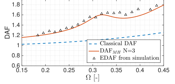
Fig. 18. DAF in reaction moment for jacket with Gumbel distribution at \alpha = 0.9 . 32 seeds at each eigenperiod. \bar{k} = [0.88, 0.15, 0.07] , \bar{\zeta} = [0.14, 0.11, 0.09]
