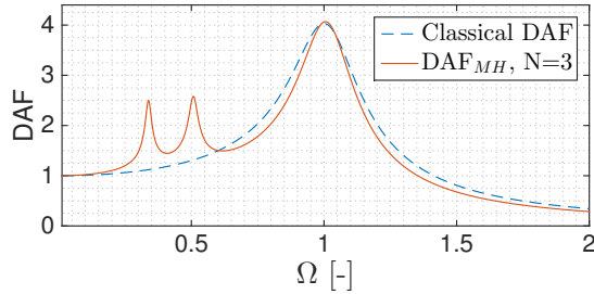
Fig. 3. Multi-harmonic DAF. \bar{k} = [0.8, 0.1, 0.1] , \bar{\zeta} = [0.10, 0.03, 0.03] .
