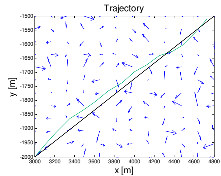
Fig. 8. Trajectory tracking result under the perturbed environment.
