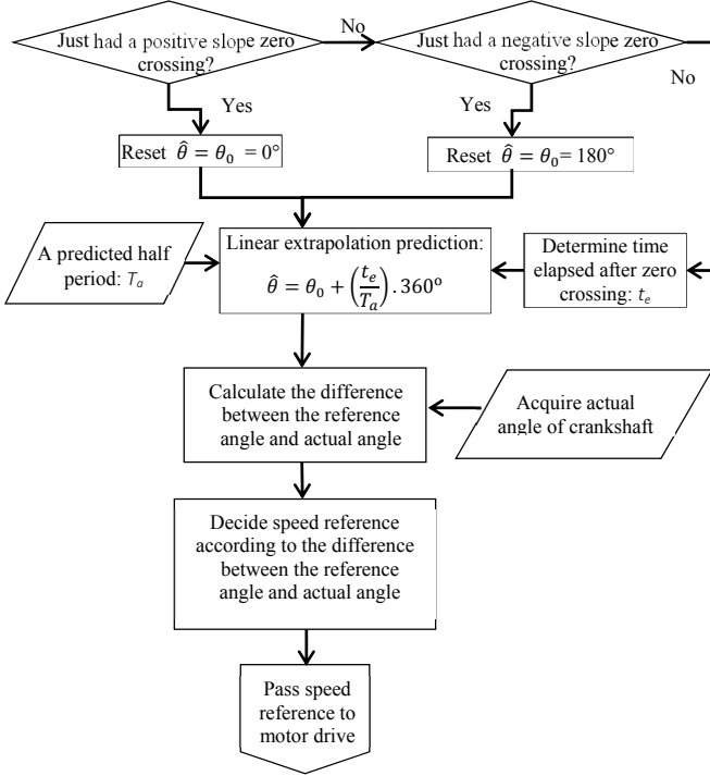
Fig. 5. Flowchart of the control algorithm
