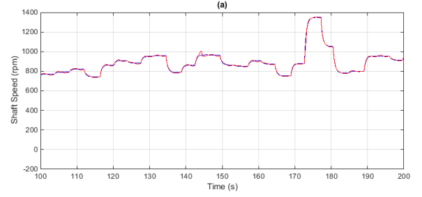
Fig. 10. Shaft speed of the AC machine
