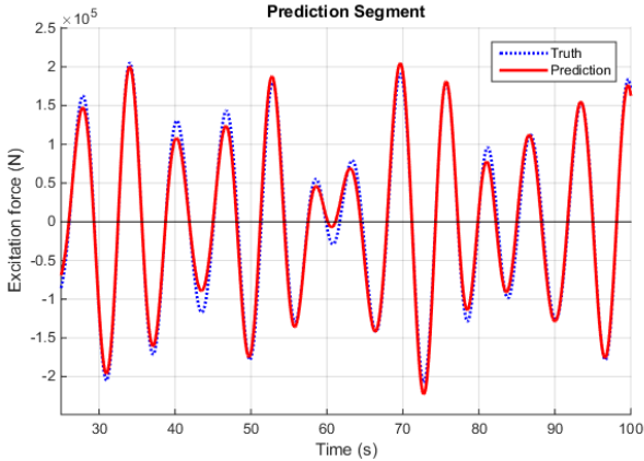
Fig. 6. Prediction of wave excitation force using the AR model
