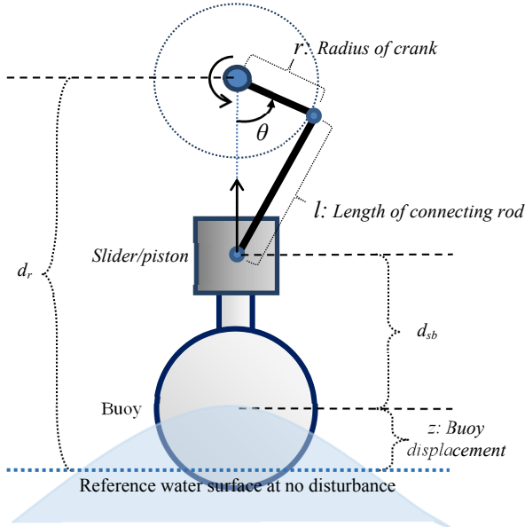
Fig. 4. Parameters of the WEC system
