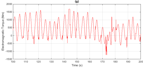
Fig. 16. Electromagnetic torque of the generator
