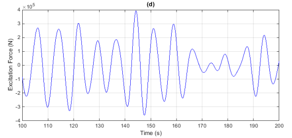
Fig. 13. Wave excitation force
