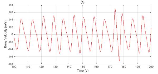
Fig. 12. Buoy velocity
