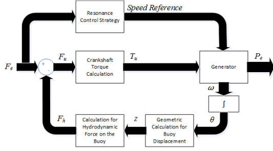
Fig. 3. Block diagram of the system
