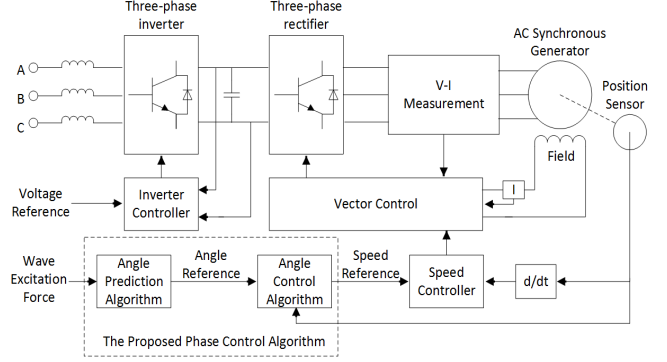
Fig. 7. Control schematics of the machine drive system
