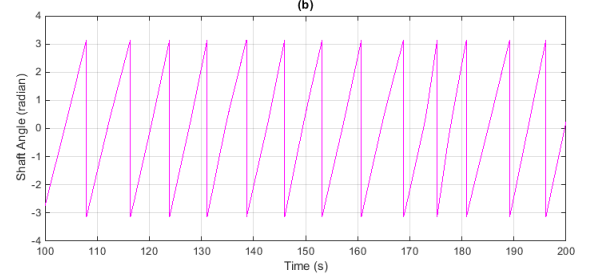
Fig. 11. Shaft angle of the AC machine
