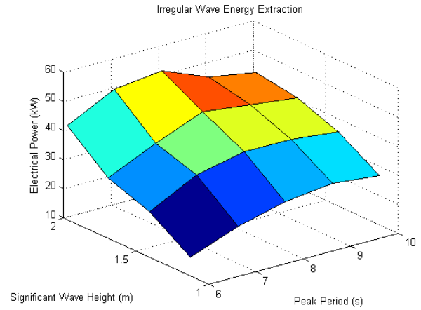
Fig. 17. Electric power production
