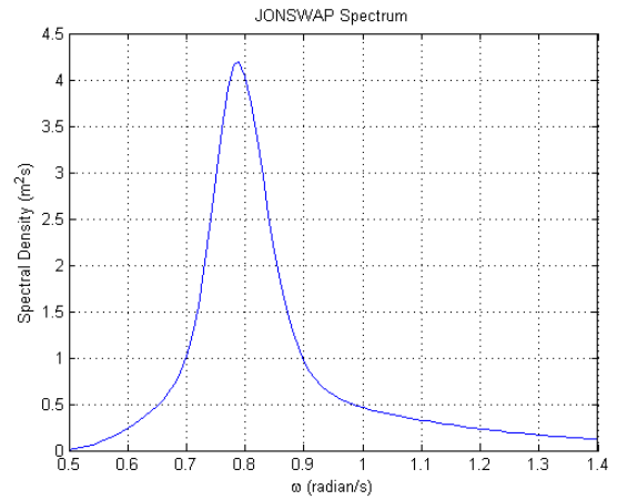
Fig. 2. An example of the JONSWAP spectrum
