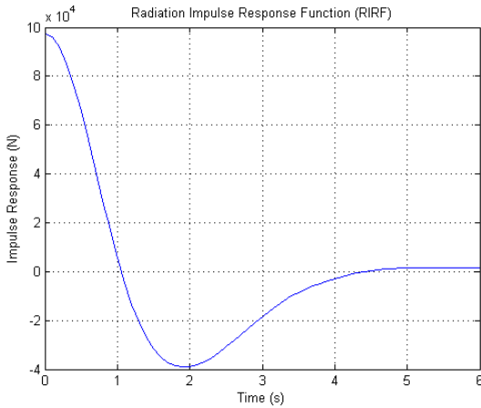
Fig. 1. Radiation impulse response function of the buoy
