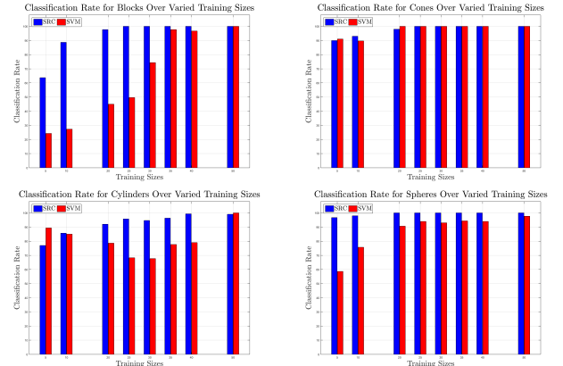
Fig. 4: Class specific classification rates over varied training.
