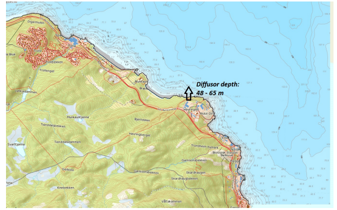
Fig. 6. Map of the Høvringen treatment plant
