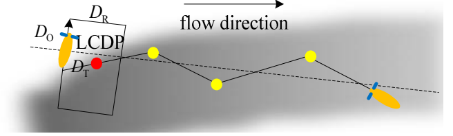
Fig. 4. Illustration of the Reacquire-Plume behavior. The dashed line represents the estimated plume centerline.
