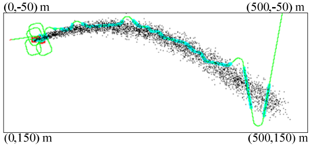
Fig. 8. A simulation result of tracking of a turbulent plume whose centerline is meandrous.
