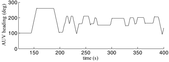
Fig. 7. AUV's heading in the plume tracing run in Fig. 5.
