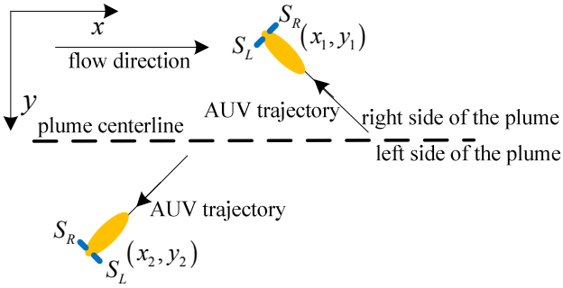
Fig. 1. Illustration of chemical plume tracing with an AUV mounted with a pair of spatially separated chemical sensors.
