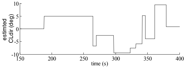
Fig. 6. Estimated direction of plume centerline in the plume tracing run in Fig. 5.
