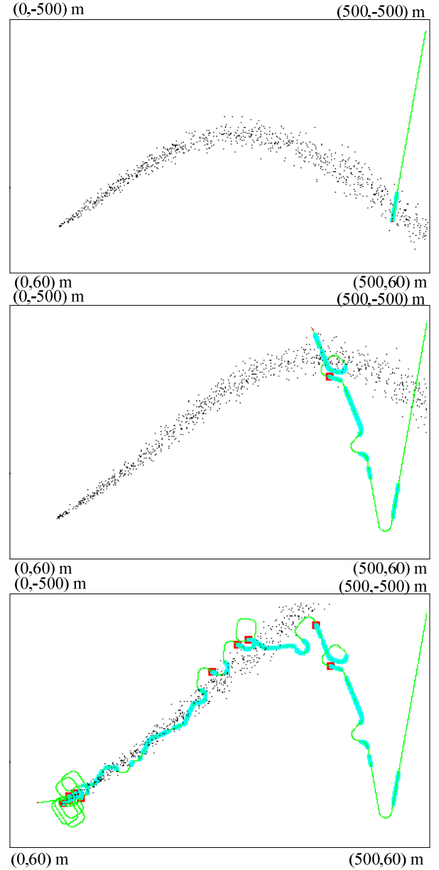
Fig. 10. A simulation result of tracking of a dynamic turbulent plume.
