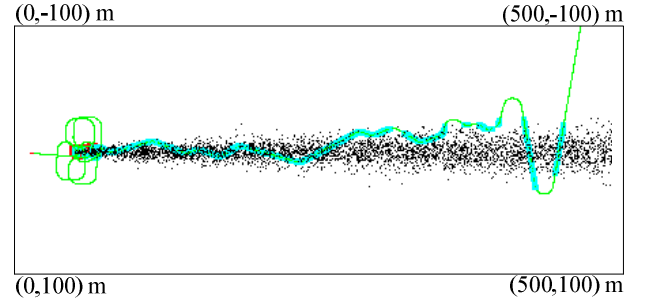
Fig. 5. A simulation result of tracking a straight turbulent plume.
