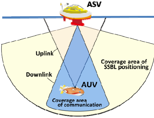
Fig. 6. Coverage areas of acoustic communication and SSBL positioning
