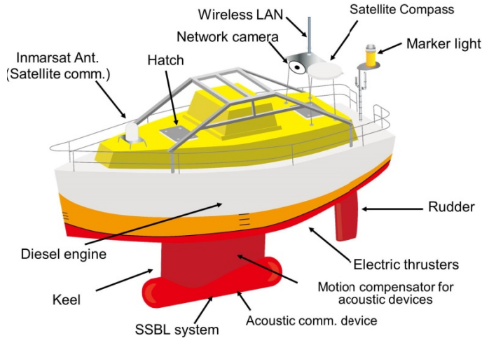
Fig. 3. General arrangement of the ASV "MAINAMI".
