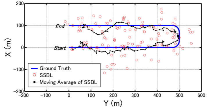
Fig. 8. Estimated trajectory by moving average of SSBL. Each measurement of SSBL is shown by a red circle. The black line shows the moving average of 10 SSBL measurements. The blue line shows the ground truth of AUV trajectory.
