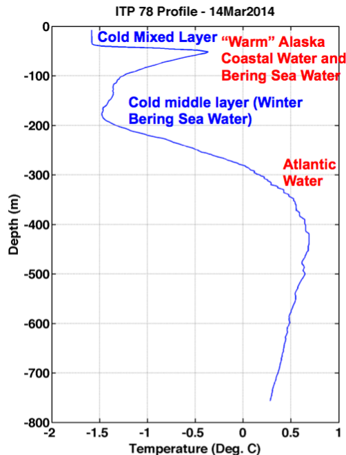
Figure 6 ITP profile showing the temperature with respect to depth and annotations with the assumed source of the different water masses.
