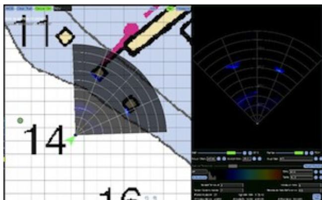
Figure 6: Typical run-time sonar and navigation display with the feature system disabled. In this mode, Greensea's interface provides a simple sonar interface with industry-wide support for forward looking sonars.
