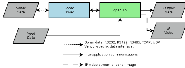
Figure 2: General feature-based system architecture.
