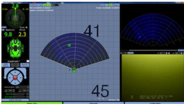
Figure 5: SeaBotix SmartFlight control interface with Greensea's feature-based navigation system utilizing a Kongsberg Mesotech M3 multibeam imaging sonar.
