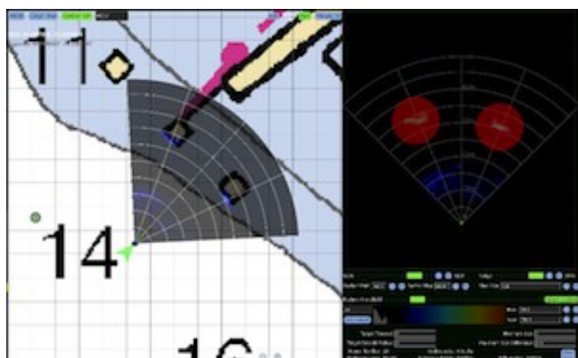
Figure 8: The openFLS feature detection module has built confidence in two of the features and has made them landmarks and pushed them into the map. The navigation module is now using these two features to correct the INS and calculate a vehicle positioning solution.
