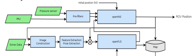
Figure 3: General architecture of Greensea's feature-based ROV navigation and positioning system.
