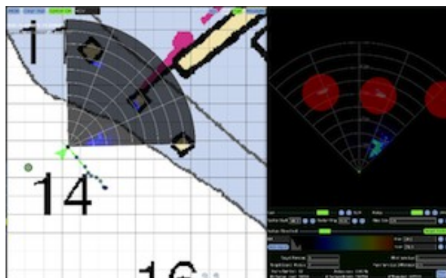
Figure 11: The new feature has become a landmark and now the system is using three landmarks to stabilize the positioning solution.
