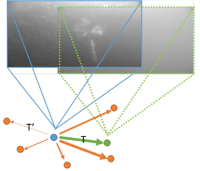
Fig. 6. This figure gives an example when a set of particles (orange dot) is associated with a single image node in a previous graph (blue dot). The transform vector T from the old graph node to the new one (green dot) is estimated in image matching. The transform vector T' from old graph node to particles are compared with T . The line weights of T' in the figure indicate the relative value of s_g in this example.
