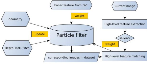
Fig. 2. System Flowchart. A particle filter is initialized on a previous SLAM graph that we will localize against. Onboard sensors including depth and IMU are used to update the particles when the vehicle is moving. Planar features estimated from DVL [6] as well as high-level features extracted from visual images are used to make measurement corrections by updating the importance weight of each particle.
