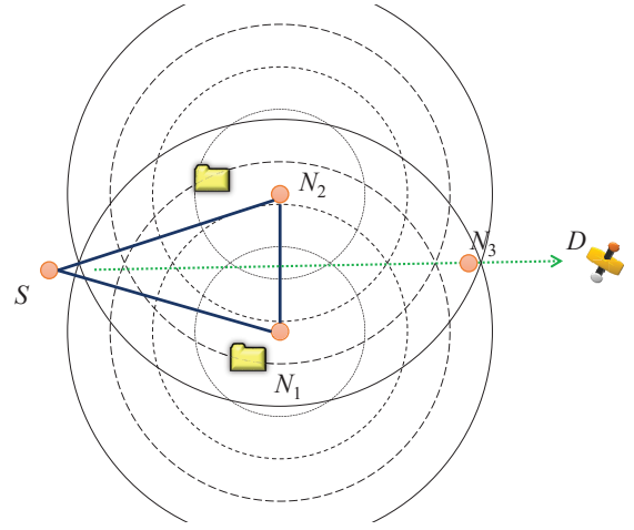
Fig. 6. The concept of cooperative line in SACRP.
