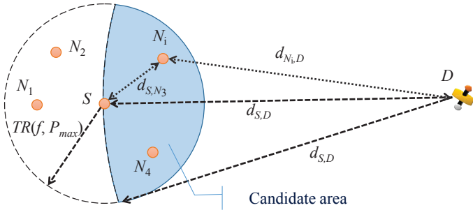
Fig. 5. The concept of candidate zone in SACRP.
