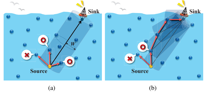
Fig. 1. The concept of (a) VBF and (b) HH-VBF Routing Protocol. Multiple routing paths work inside the pipe to increase the robustness of DATA delivery.
