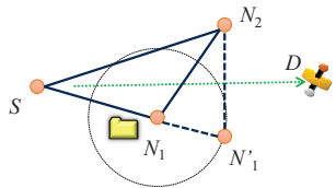
Fig. 7. The concept of cooperation timing decision in SACRP.
