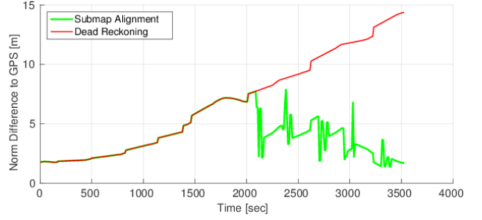
(a) Norm difference between estimated poses to GPS optimized graph
