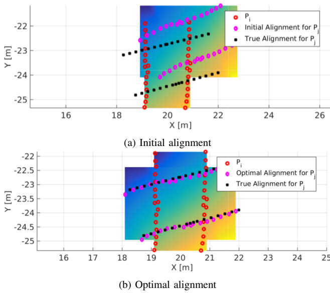
Fig. 3: Top view of submap alignment results in simulation. The top figure shows the initial condition alignment (pink) versus the correct alignment (black). The bottom figure shows the optimized submap alignment (pink) matching the correct alignment (black). Red is the submap of the first node.
