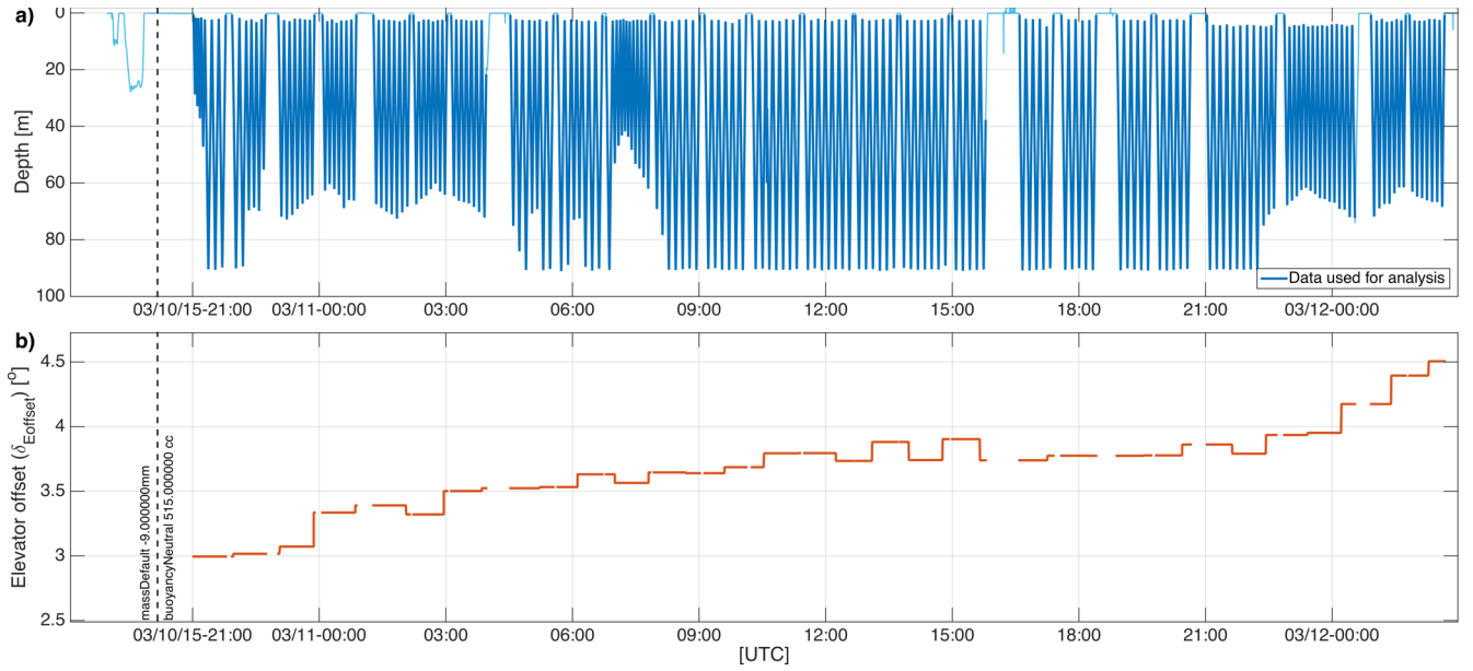
Fig. 5. (a) Depth record from the Daphne LRAUV test in Monterey Bay in March 2015. Only data collected during flight mode (shown dark blue) is considered for analysis. (b) Time series of the calculated offset angle of the stern plane control surface (orange). Once ballast and trim configuration is set (black dashed vertical line), the offset is expected to persist; in this dataset an upward trend can clearly be seen.
