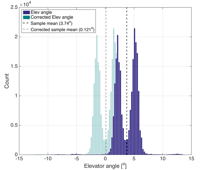
Fig. 2. Histogram of elevator angles recorded by the Daphne LRAUV in February 2015 while on a yo-yo trajectory (in flight mode; shown in dark blue). The repetitive descent-ascent cycles of the yo-yo profile yield a symmetric bimodal distribution. The elevator offset \delta_{E_{offset}} is approximated as given in (1) (dark dashed line). The corrected data (offset removed) is shown in light blue.
