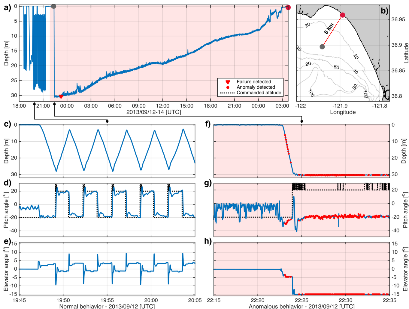
Fig. 1. Depth (panels a, c and f), pitch angle (d and g), and elevator angle (e and h) measurements from the Tethys LRAUV bottoming incident that took place on September 12 to September 14, 2013 in Monterey Bay. The grey circle in panels a and b mark the time and location of the AUV's last decent before bottoming. The AUV descended at extreme pitch angles and was unable change its attitude (bottom right panels f-h). After bottoming the AUV's fault detection and failure prevention system identified the problem as a vertical control failure at 23:15 UTC (red triangle in panel a). The AUV remained underwater for 27 hours until recovered on the beach 8 km away from its original position (red circle in panels a and b). In post-processing tests the newly developed detector identified the anomaly ~1 minute after the AUV began its final decent (red dots in bottom right panels f-h). An example of the AUV's expected vertical plane performance recorded prior to the bottoming incident is also shown (bottom left panels b-e).
