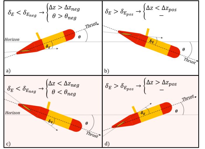
Fig. 3. Illustration of an LRAUV in flight mode. The top panels a, and b provide an example of "normal" vertical plane performance; in both panels the state parameters \delta_E , \Delta z and \theta do not violate the conditional tests, or in other words, the "response" matches the AUV's "intention". Conversely, panels c, and d depict anomalous performance where the state parameters \delta_E , \Delta z and \theta violate the conditional tests. For example, in (c) the vehicle has set its elevators to pull up, but remains nose down.
