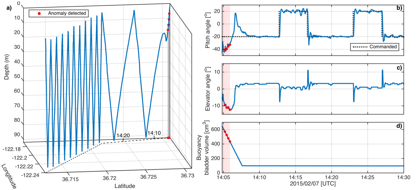
Fig. 4. (a) Depth record from a segment of the AUV's transect during February 2015 test in Monterey Bay. Also shown in close-up are the AUV's measurements of: pitch angle in (b), elevator angle in (c), and buoyancy bladder volume in (d). The times and locations where the AUV determined it was experiencing a vertical plane flight anomaly are marked by red dots (over red background). After the buoyancy package was sufficiently emptied ( \sim 410 \text{ cm}^3 ) the AUV regained vertical control and returned to normal performance.
